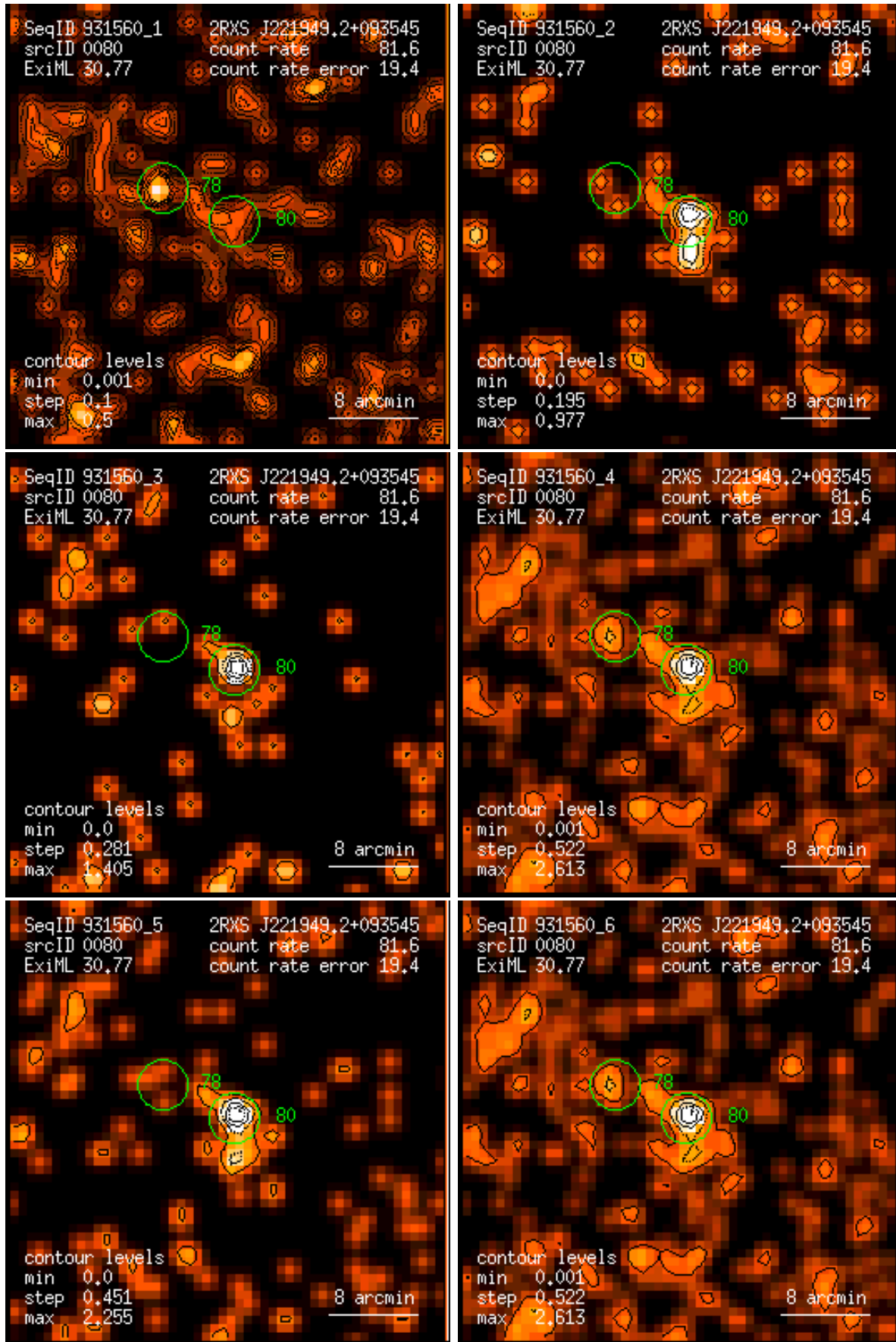
Figure 80: RASS 931560: detection 0080: band rate images, Gaussian filter: (1) PSPC channels 11 – 41, (2) 52 – 90, (3) 91 – 201, (4) 11 – 235, (5) 52 – 201, (6) 11 – 201. Broad band rates in counts/ks. Band rate contour levels in counts/ks/arcmin 2 .
