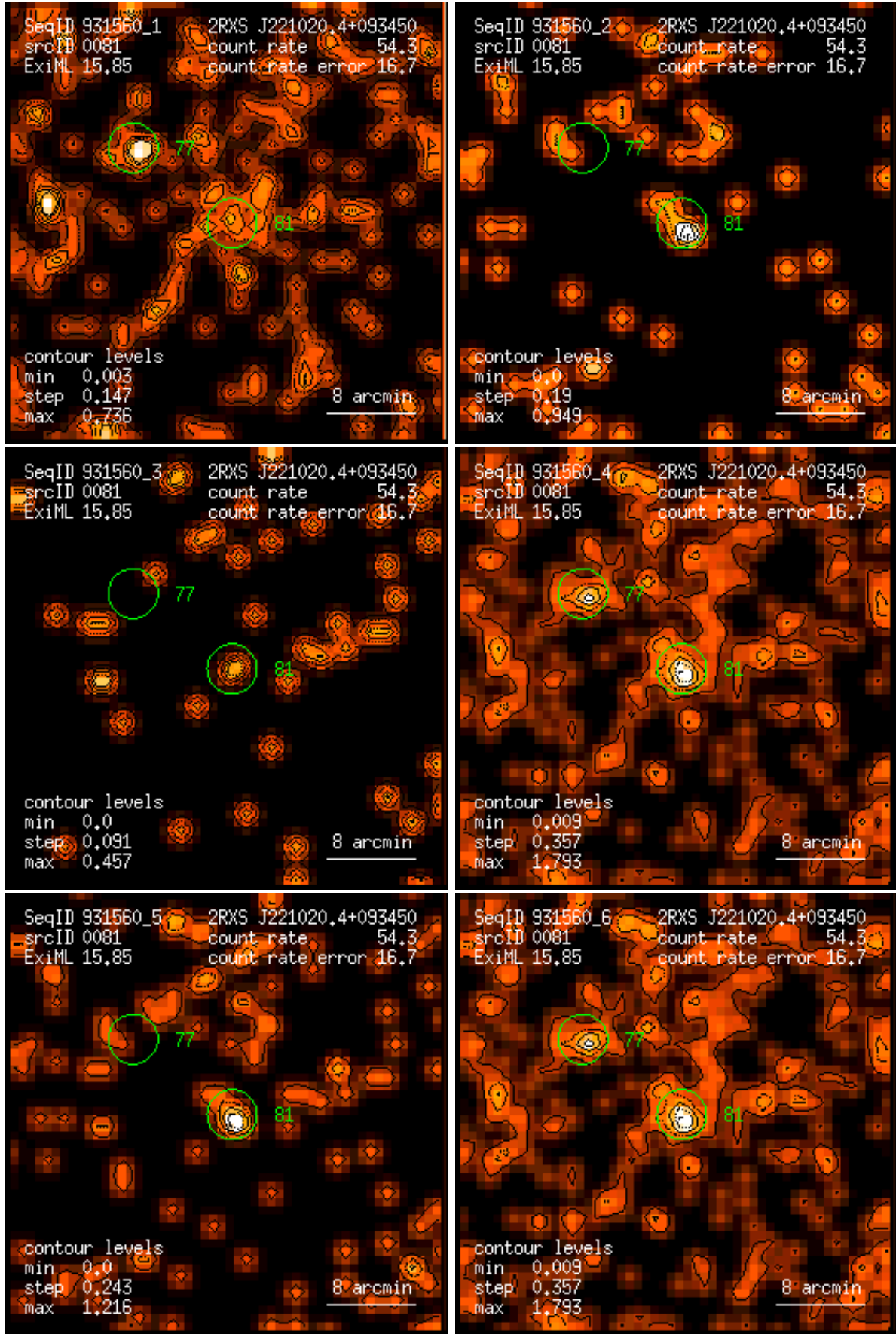
Figure 81: RASS 931560: detection 0081: band rate images, Gaussian filter: (1) PSPC channels 11 – 41, (2) 52 – 90, (3) 91 – 201, (4) 11 – 235, (5) 52 – 201, (6) 11 – 201. Broad band rates in counts/ks. Band rate contour levels in counts/ks/arcmin 2 .
