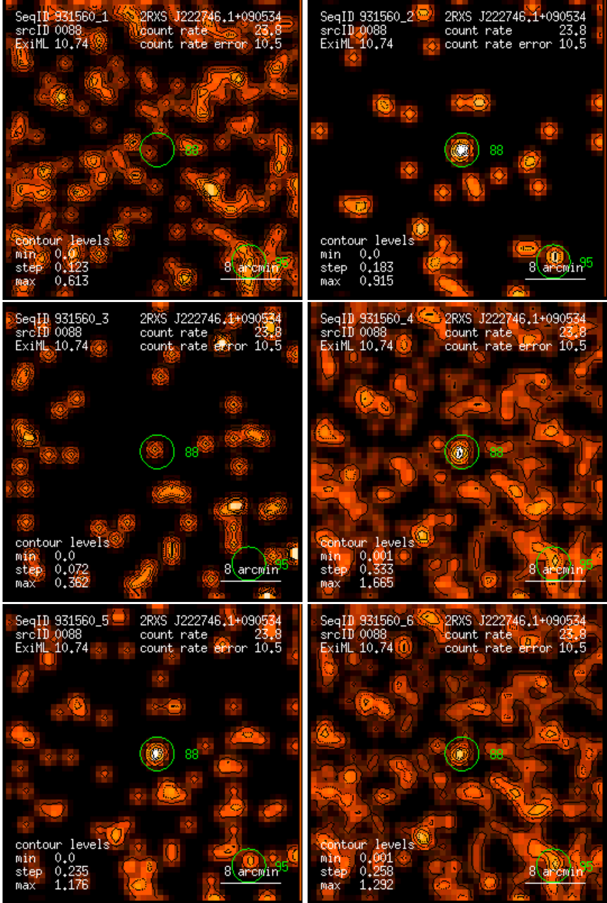
Figure 88: RASS 931560: detection 0088: band rate images, Gaussian filter: (1) PSPC channels 11 – 41, (2) 52 – 90, (3) 91 – 201, (4) 11 – 235, (5) 52 – 201, (6) 11 – 201. Broad band rates in counts/ks. Band rate contour levels in counts/ks/arcmin 2 .
