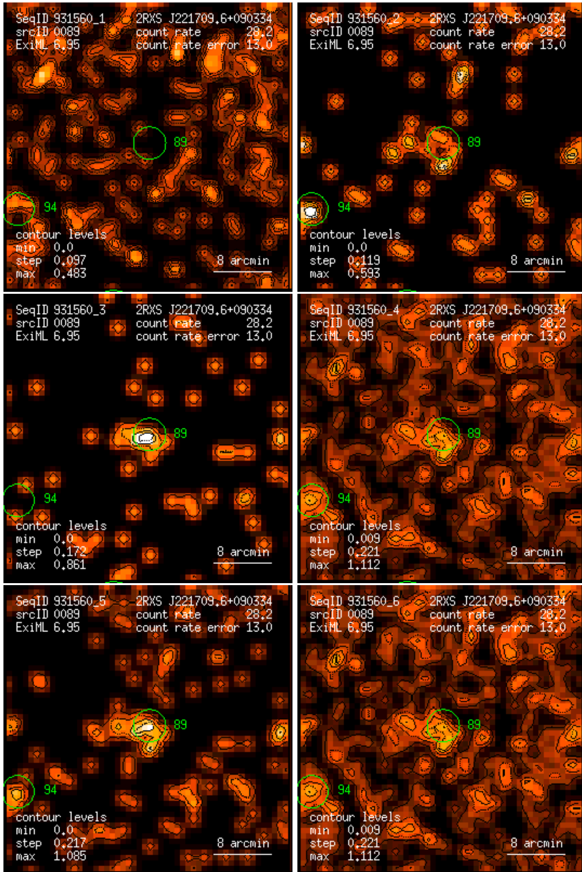
Figure 89: RASS 931560: detection 0089: band rate images, Gaussian filter: (1) PSPC channels 11 – 41, (2) 52 – 90, (3) 91 – 201, (4) 11 – 235, (5) 52 – 201, (6) 11 – 201. Broad band rates in counts/ks. Band rate contour levels in counts/ks/arcmin 2 .
