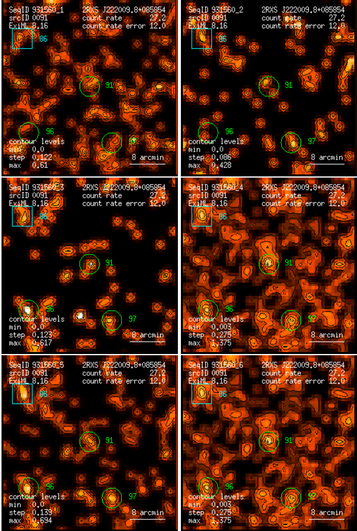
Figure 91: RASS 931560: detection 0091: band rate images, Gaussian filter: (1) PSPC channels 11 – 41, (2) 52 – 90, (3) 91 – 201, (4) 11 – 235, (5) 52 – 201, (6) 11 – 201. Broad band rates in counts/ks. Band rate contour levels in counts/ks/arcmin 2 .
