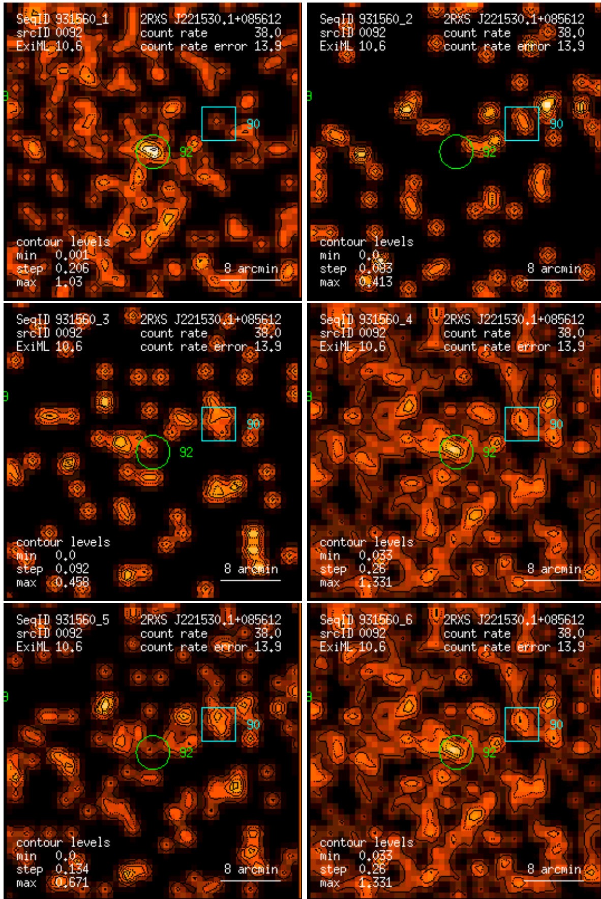
Figure 92: RASS 931560: detection 0092: band rate images, Gaussian filter: (1) PSPC channels 11 – 41, (2) 52 – 90, (3) 91 – 201, (4) 11 – 235, (5) 52 – 201, (6) 11 – 201. Broad band rates in counts/ks. Band rate contour levels in counts/ks/arcmin 2 .
