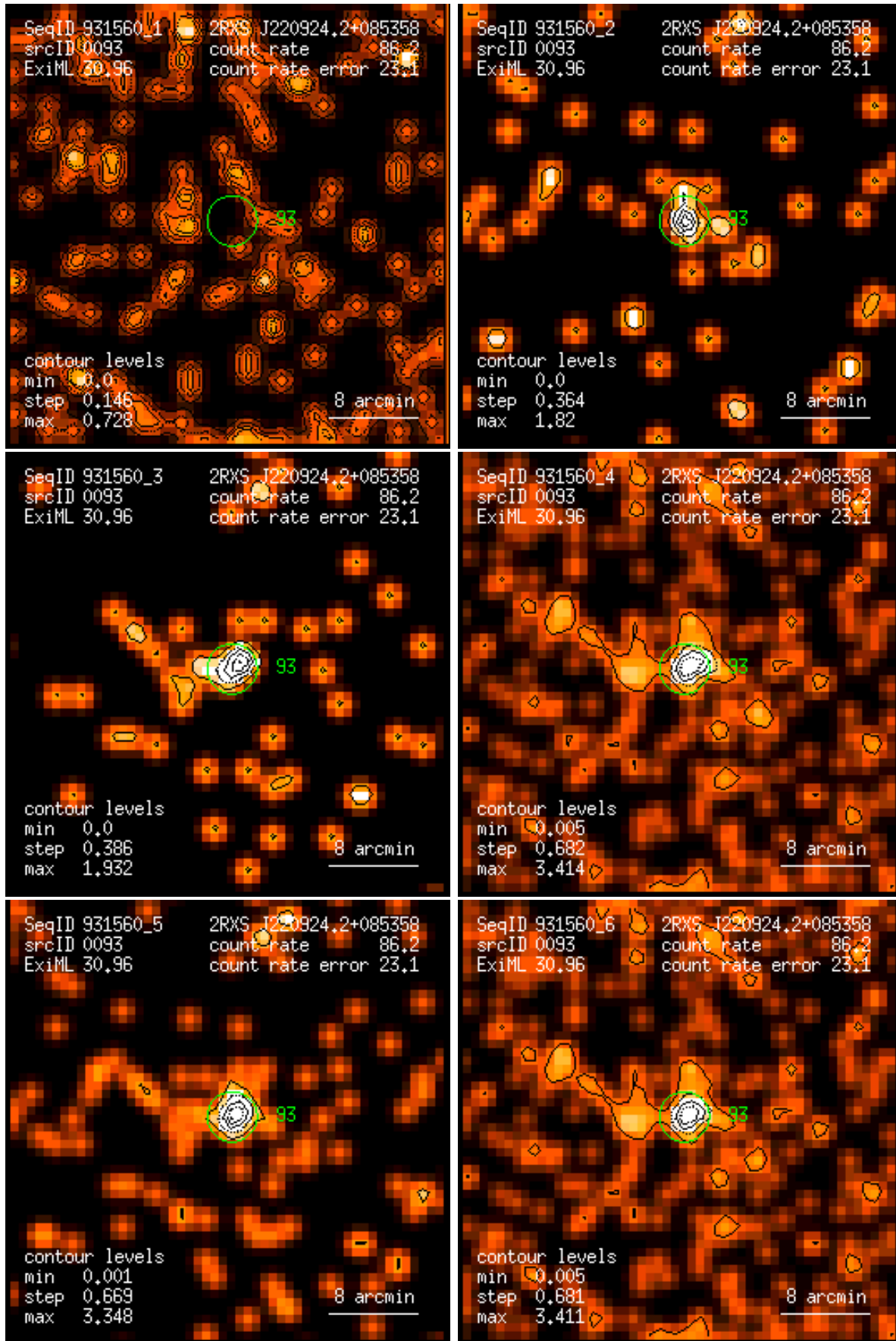
Figure 93: RASS 931560: detection 0093: band rate images, Gaussian filter: (1) PSPC channels 11 – 41, (2) 52 – 90, (3) 91 – 201, (4) 11 – 235, (5) 52 – 201, (6) 11 – 201. Broad band rates in counts/ks. Band rate contour levels in counts/ks/arcmin 2 .
