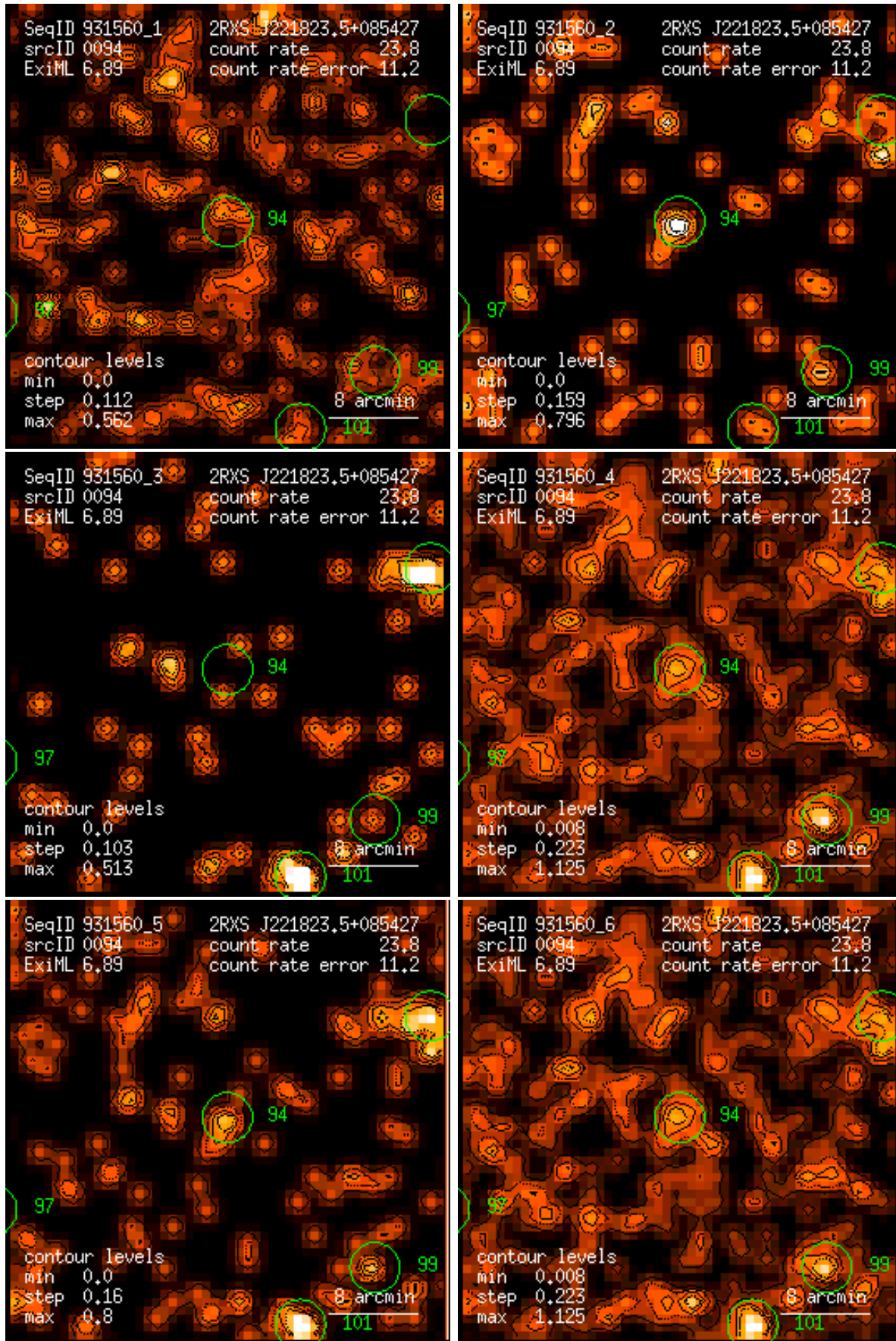
Figure 94: RASS 931560: detection 0094: band rate images, Gaussian filter: (1) PSPC channels 11 – 41, (2) 52 – 90, (3) 91 – 201, (4) 11 – 235, (5) 52 – 201, (6) 11 – 201. Broad band rates in counts/ks. Band rate contour levels in counts/ks/arcmin 2 .
