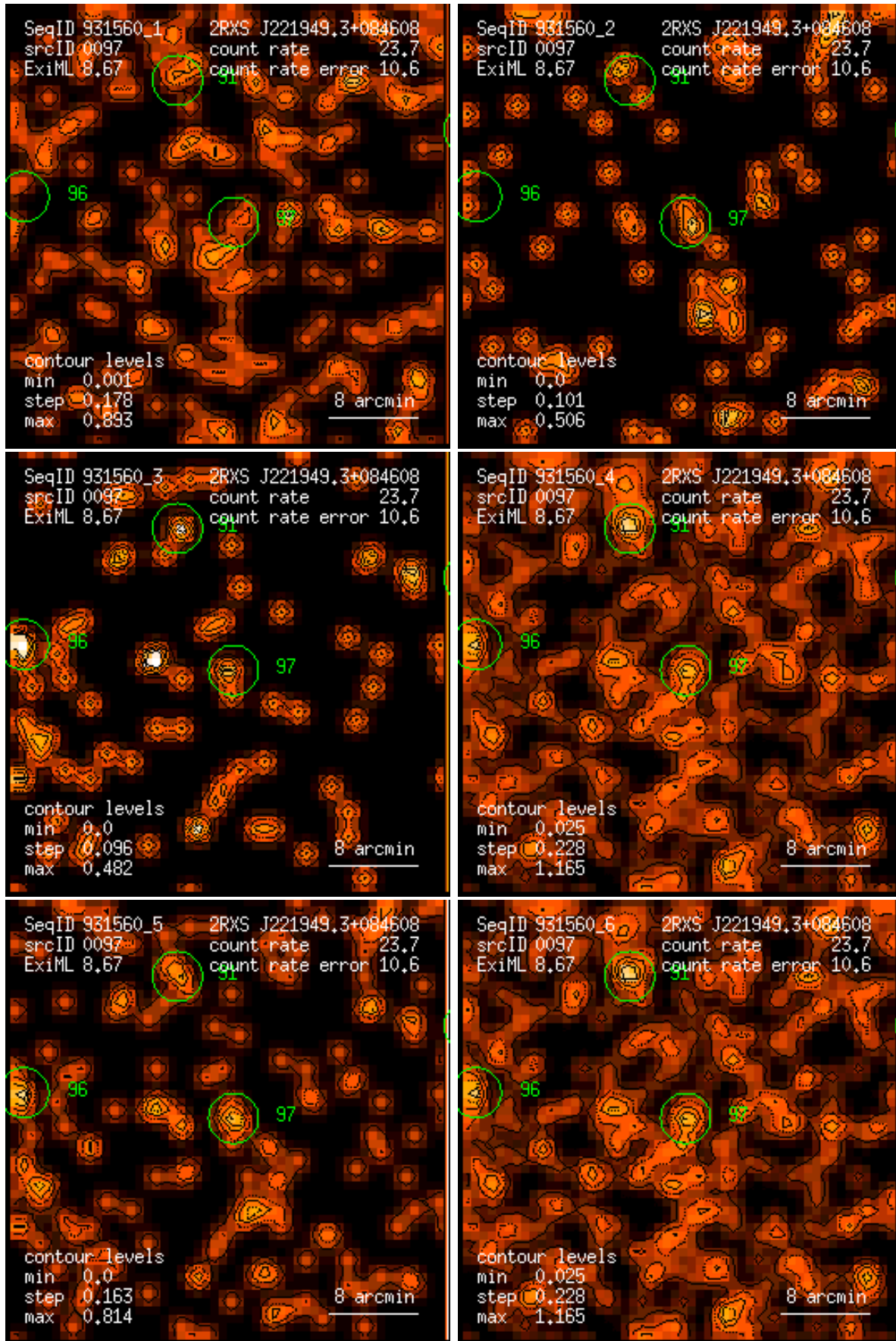
Figure 97: RASS 931560: detection 0097: band rate images, Gaussian filter: (1) PSPC channels 11 – 41, (2) 52 – 90, (3) 91 – 201, (4) 11 – 235, (5) 52 – 201, (6) 11 – 201. Broad band rates in counts/ks. Band rate contour levels in counts/ks/arcmin 2 .
