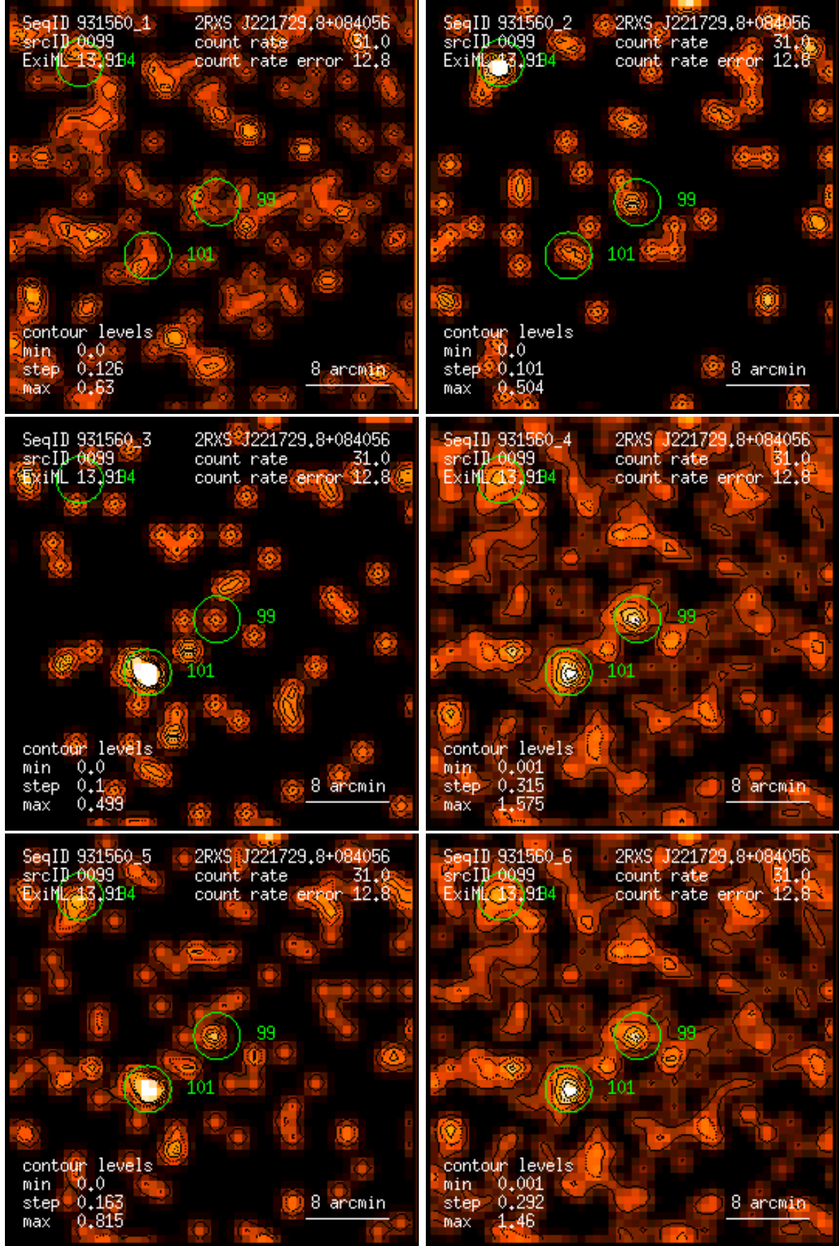
Figure 99: RASS 931560: detection 0099: band rate images, Gaussian filter: (1) PSPC channels 11 – 41, (2) 52 – 90, (3) 91 – 201, (4) 11 – 235, (5) 52 – 201, (6) 11 – 201. Broad band rates in counts/ks. Band rate contour levels in counts/ks/arcmin 2 .
