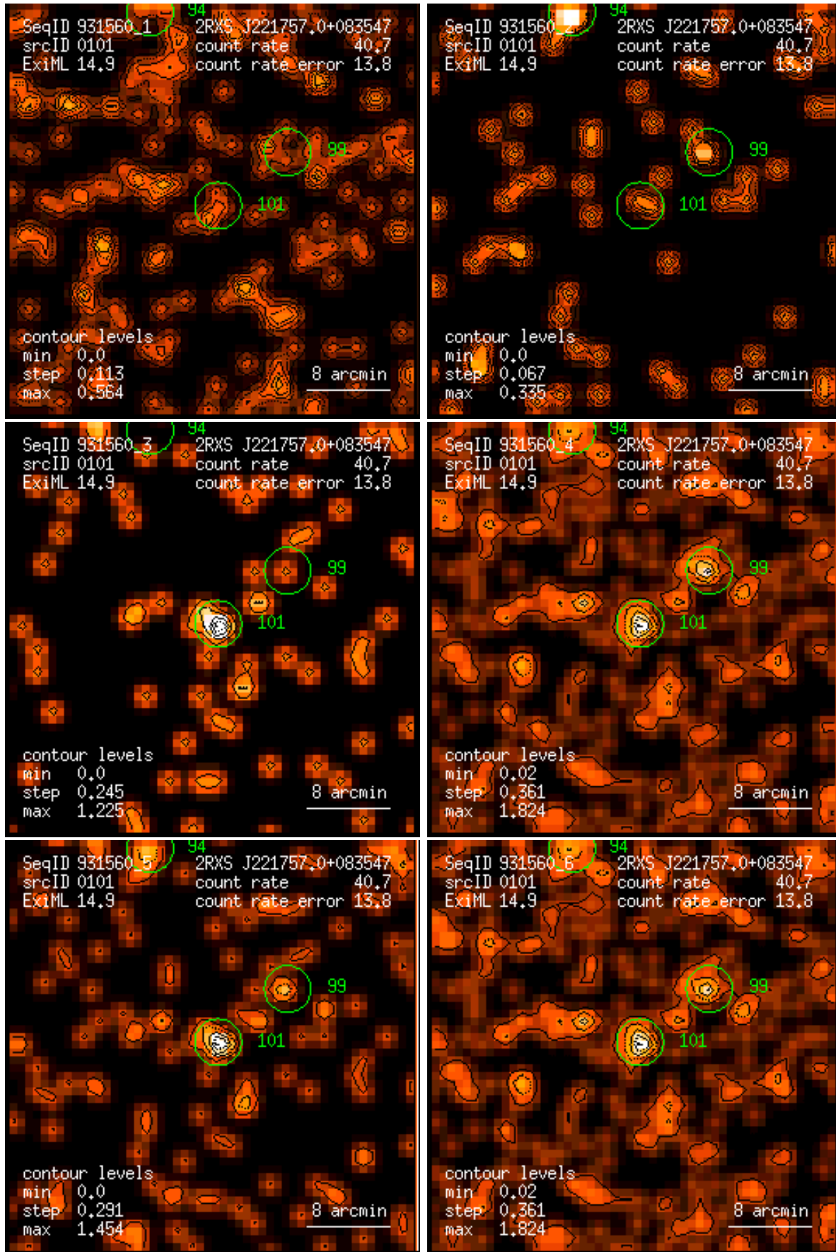
Figure 101: RASS 931560: detection 0101: band rate images, Gaussian filter: (1) PSPC channels 11 – 41, (2) 52 – 90, (3) 91 – 201, (4) 11 – 235, (5) 52 – 201, (6) 11 – 201. Broad band rates in counts/ks. Band rate contour levels in counts/ks/arcmin 2 .
