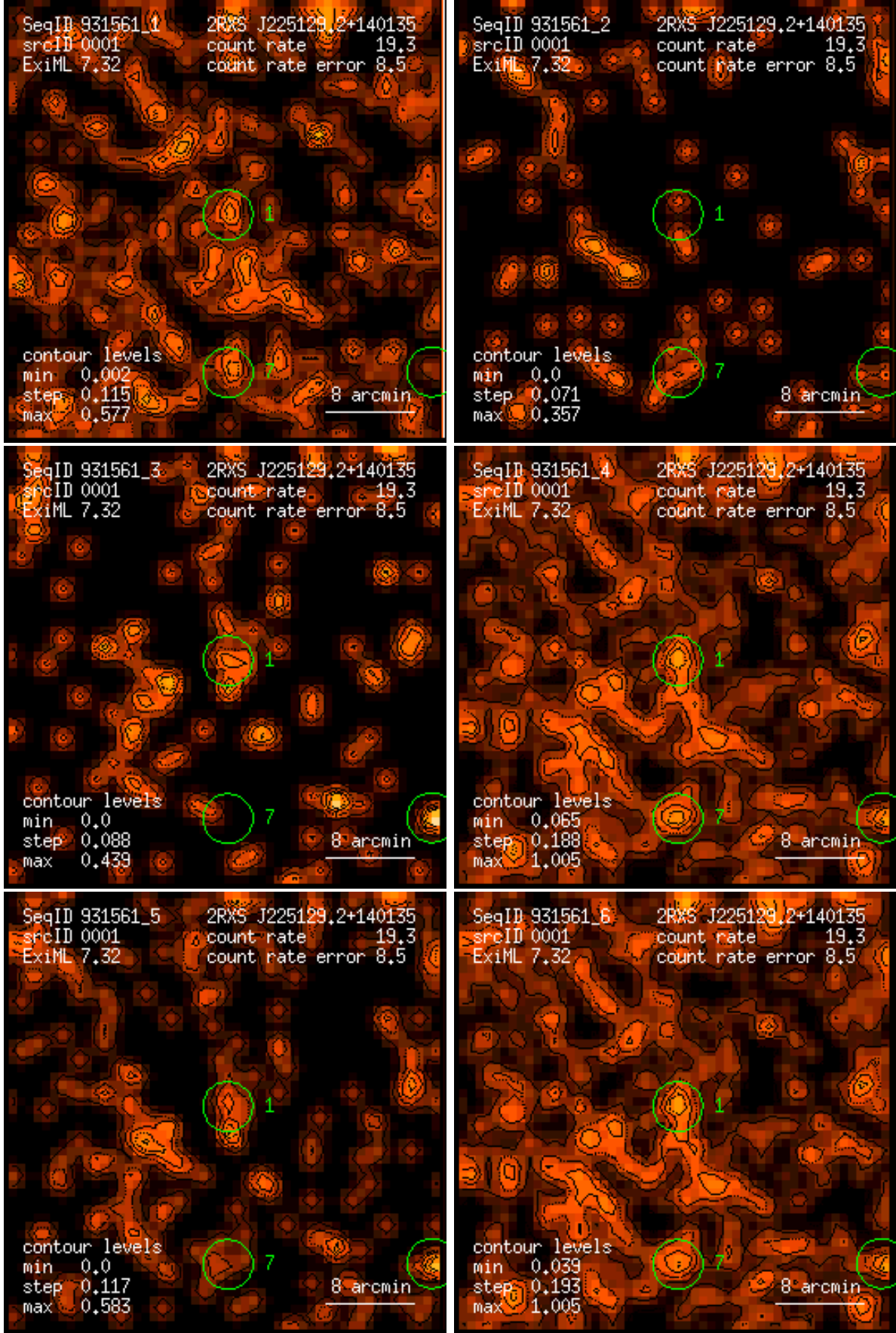
Figure 1: RASS 931561: detection 0001: band rate images, Gaussian filter: (1) PSPC channels 11 – 41, (2) 52 – 90, (3) 91 – 201, (4) 11 – 235, (5) 52 – 201, (6) 11 – 201. Broad band rates in counts/ks. Band rate contour levels in counts/ks/arcmin 2 .
