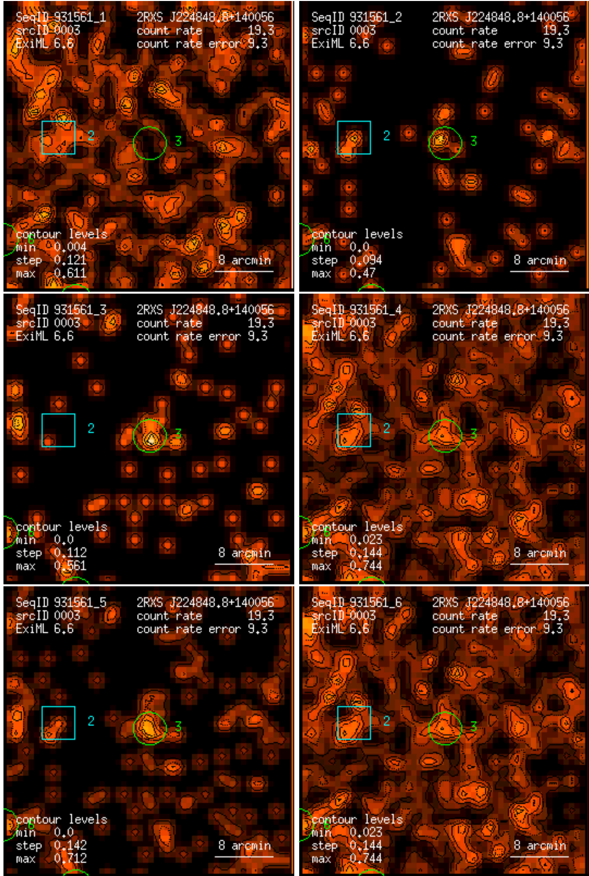
Figure 3: RASS 931561: detection 0003: band rate images, Gaussian filter: (1) PSPC channels 11 – 41, (2) 52 – 90, (3) 91 – 201, (4) 11 – 235, (5) 52 – 201, (6) 11 – 201. Broad band rates in counts/ks. Band rate contour levels in counts/ks/arcmin 2 .
