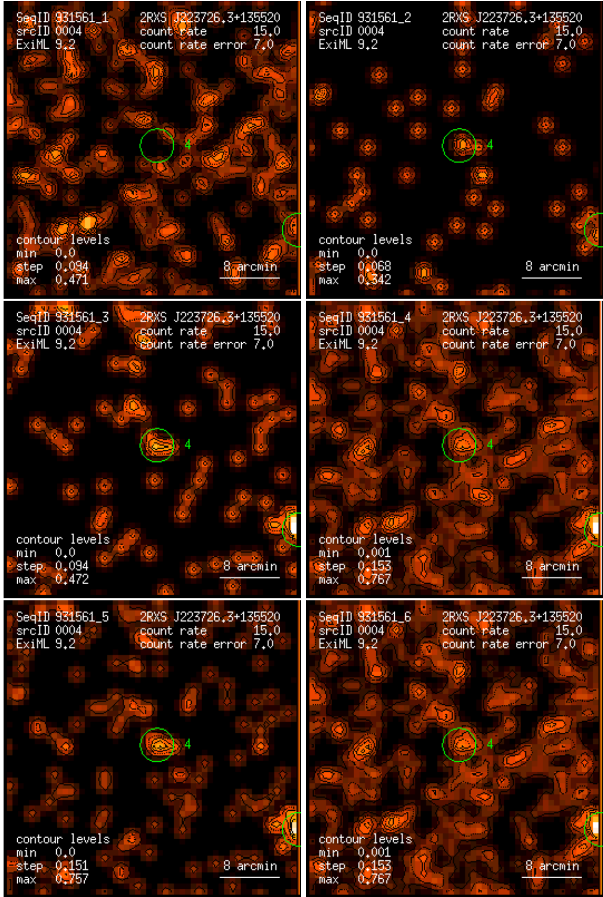
Figure 4: RASS 931561: detection 0004: band rate images, Gaussian filter: (1) PSPC channels 11 – 41, (2) 52 – 90, (3) 91 – 201, (4) 11 – 235, (5) 52 – 201, (6) 11 – 201. Broad band rates in counts/ks. Band rate contour levels in counts/ks/arcmin 2 .
