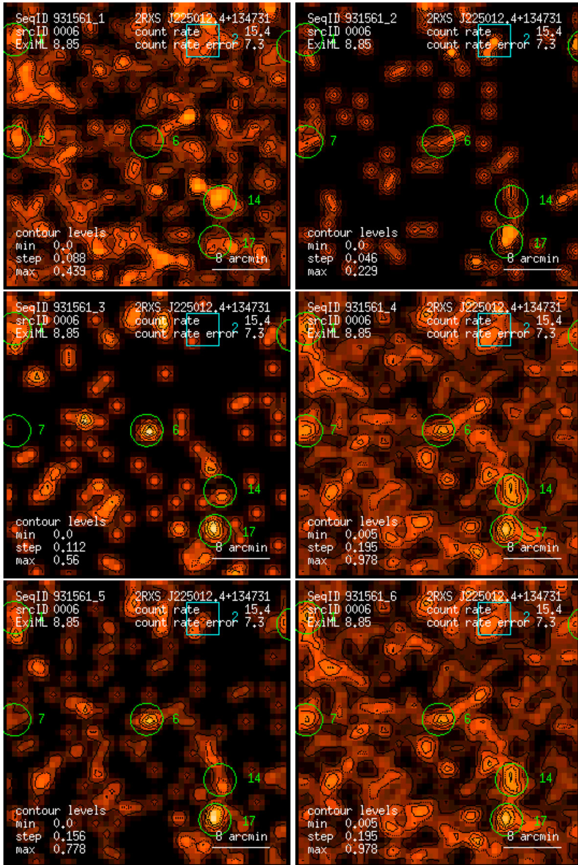
Figure 6: RASS 931561: detection 0006: band rate images, Gaussian filter: (1) PSPC channels 11 – 41, (2) 52 – 90, (3) 91 – 201, (4) 11 – 235, (5) 52 – 201, (6) 11 – 201. Broad band rates in counts/ks. Band rate contour levels in counts/ks/arcmin 2 .
