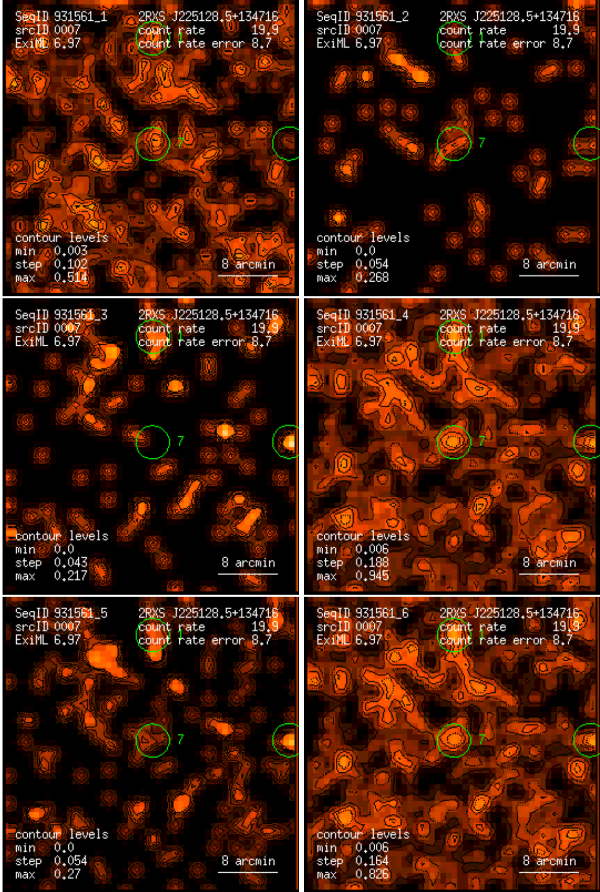
Figure 7: RASS 931561: detection 0007: band rate images, Gaussian filter: (1) PSPC channels 11 – 41, (2) 52 – 90, (3) 91 – 201, (4) 11 – 235, (5) 52 – 201, (6) 11 – 201. Broad band rates in counts/ks. Band rate contour levels in counts/ks/arcmin 2 .
