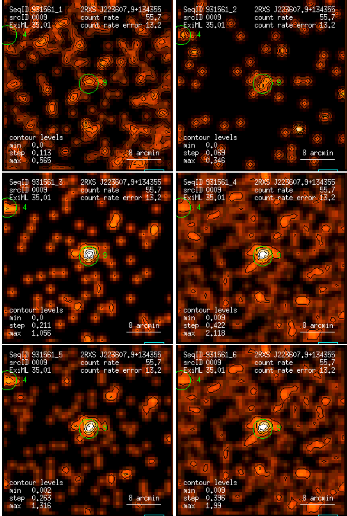
Figure 9: RASS 931561: detection 0009: band rate images, Gaussian filter: (1) PSPC channels 11 – 41, (2) 52 – 90, (3) 91 – 201, (4) 11 – 235, (5) 52 – 201, (6) 11 – 201. Broad band rates in counts/ks. Band rate contour levels in counts/ks/arcmin 2 .
