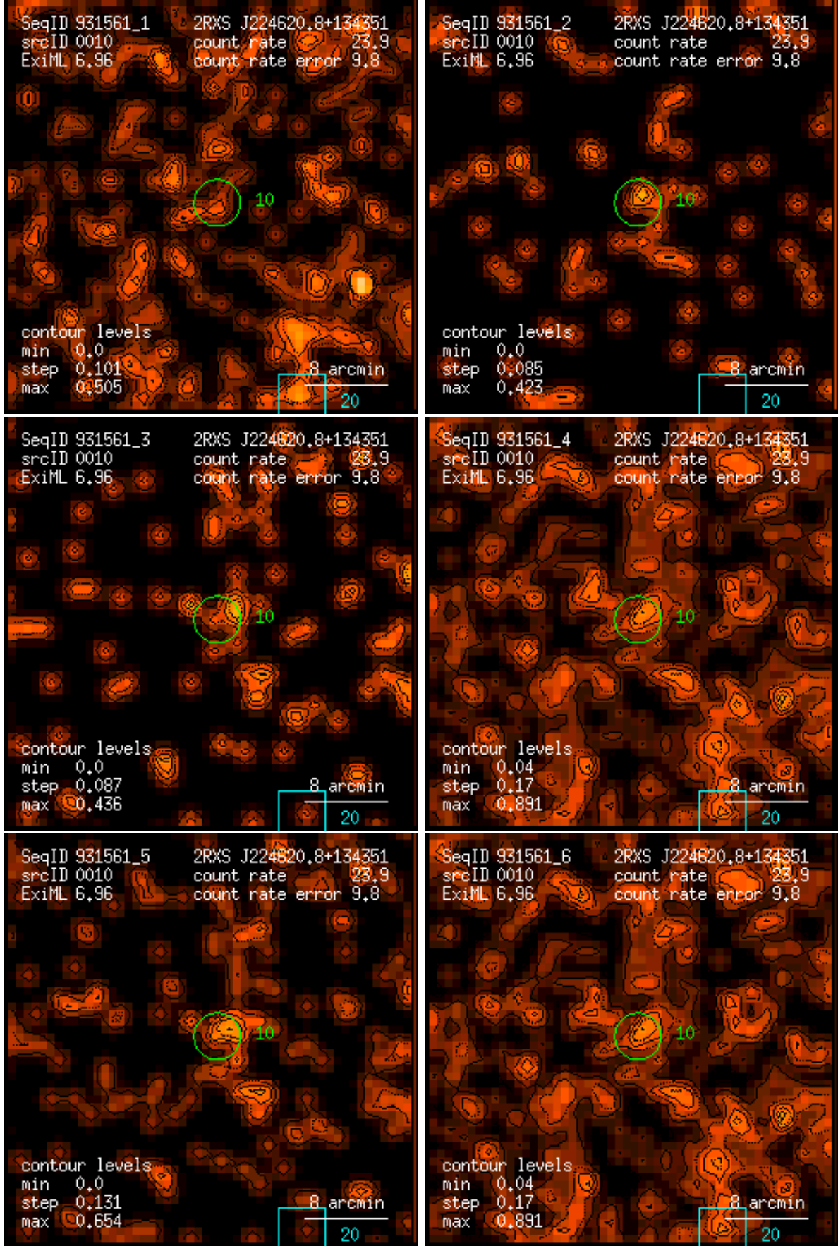
Figure 10: RASS 931561: detection 0010: band rate images, Gaussian filter: (1) PSPC channels 11 – 41, (2) 52 – 90, (3) 91 – 201, (4) 11 – 235, (5) 52 – 201, (6) 11 – 201. Broad band rates in counts/ks. Band rate contour levels in counts/ks/arcmin 2 .
