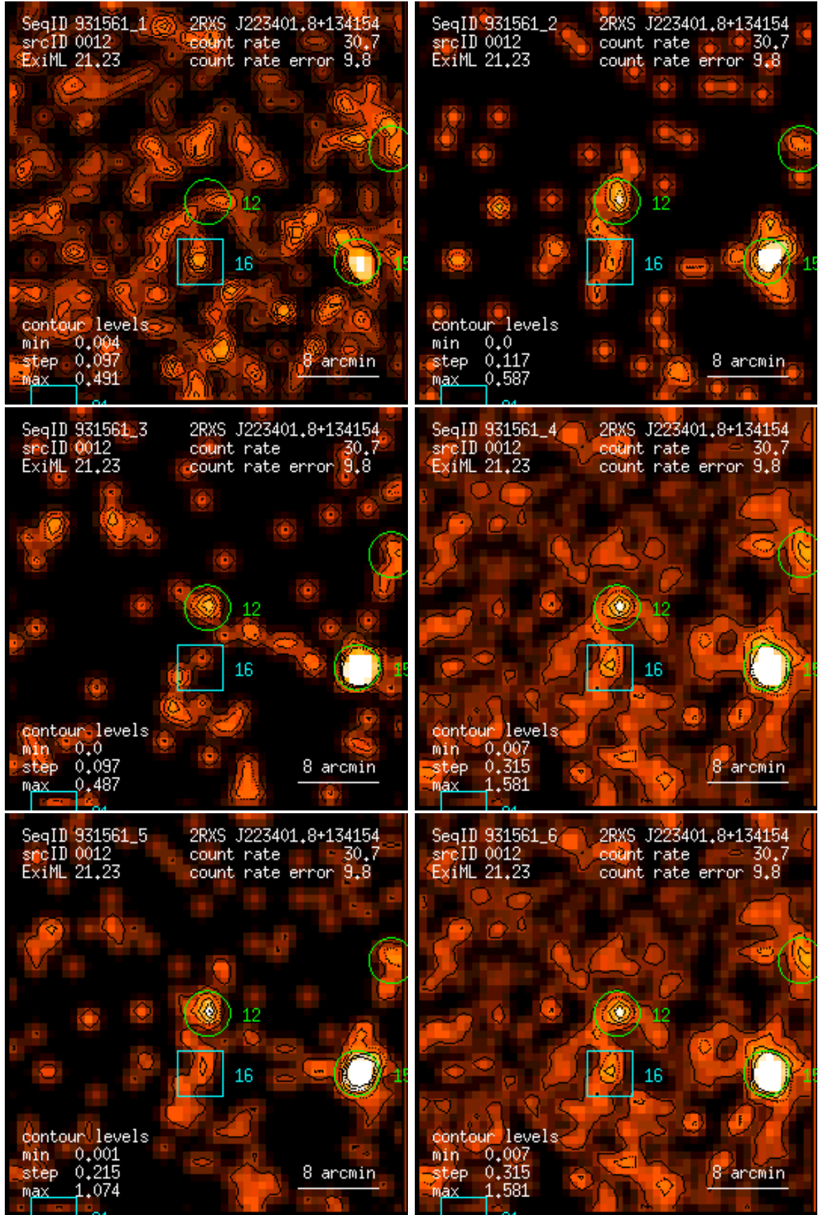
Figure 12: RASS 931561: detection 0012: band rate images, Gaussian filter: (1) PSPC channels 11 – 41, (2) 52 – 90, (3) 91 – 201, (4) 11 – 235, (5) 52 – 201, (6) 11 – 201. Broad band rates in counts/ks. Band rate contour levels in counts/ks/arcmin 2 .
