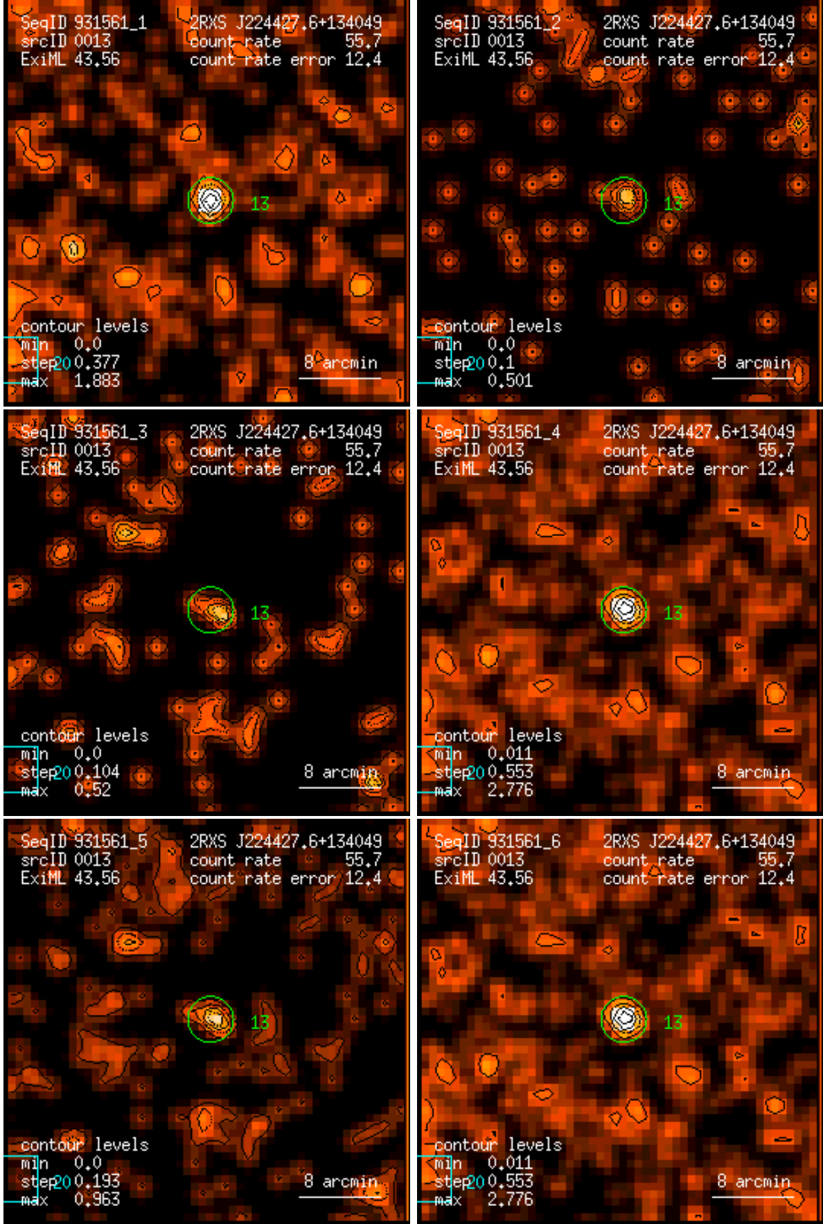
Figure 13: RASS 931561: detection 0013: band rate images, Gaussian filter: (1) PSPC channels 11 – 41, (2) 52 – 90, (3) 91 – 201, (4) 11 – 235, (5) 52 – 201, (6) 11 – 201. Broad band rates in counts/ks. Band rate contour levels in counts/ks/arcmin 2 .
