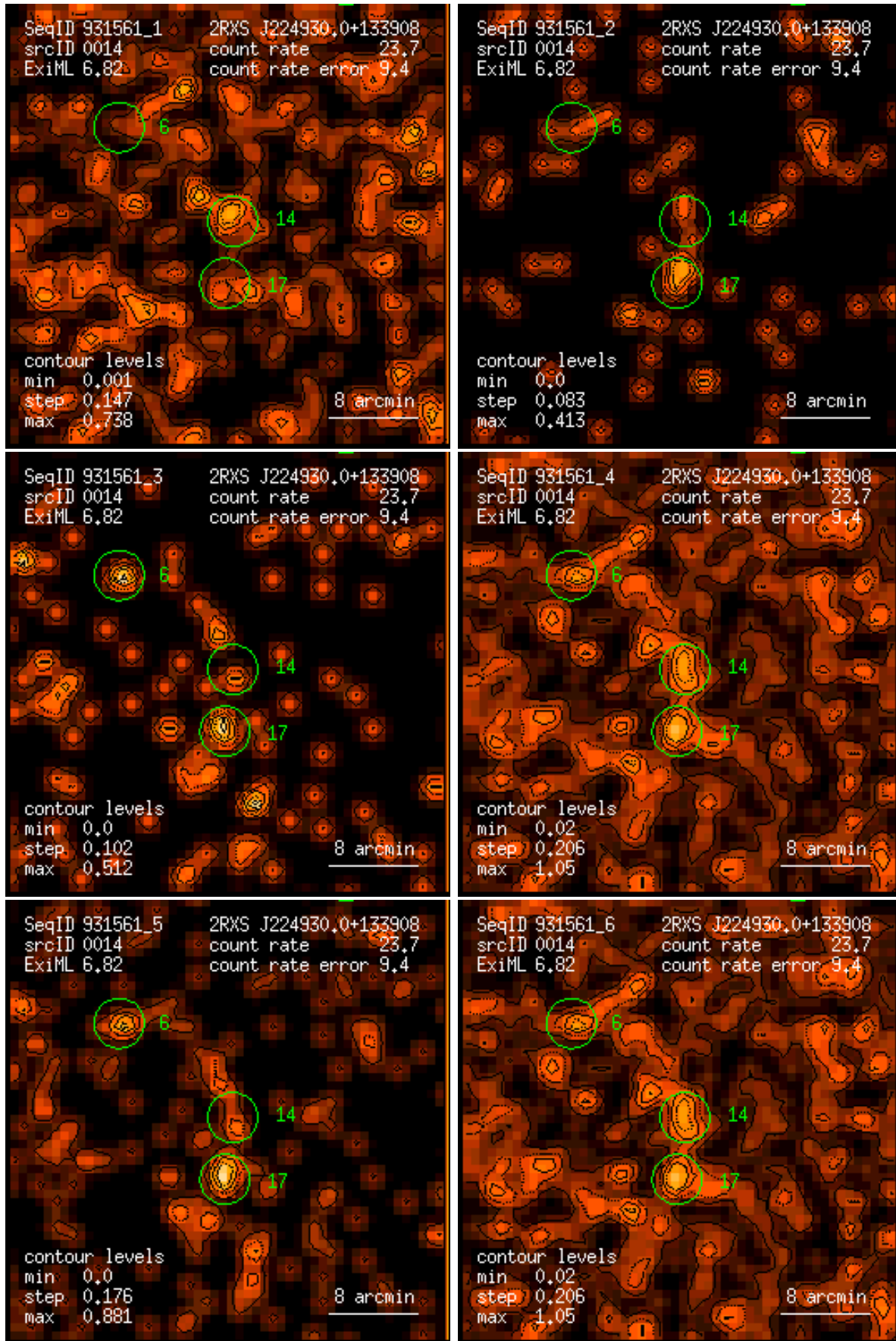
Figure 14: RASS 931561: detection 0014: band rate images, Gaussian filter: (1) PSPC channels 11 – 41, (2) 52 – 90, (3) 91 – 201, (4) 11 – 235, (5) 52 – 201, (6) 11 – 201. Broad band rates in counts/ks. Band rate contour levels in counts/ks/arcmin 2 .
