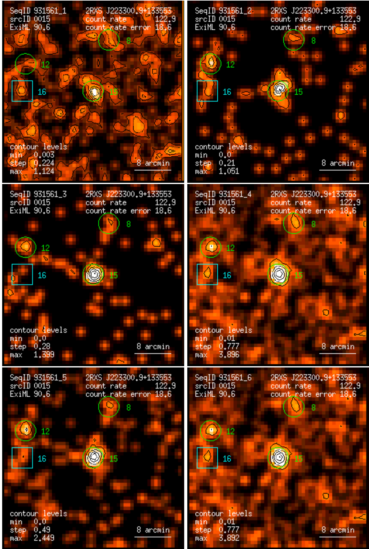
Figure 15: RASS 931561: detection 0015: band rate images, Gaussian filter: (1) PSPC channels 11 – 41, (2) 52 – 90, (3) 91 – 201, (4) 11 – 235, (5) 52 – 201, (6) 11 – 201. Broad band rates in counts/ks. Band rate contour levels in counts/ks/arcmin 2 .
