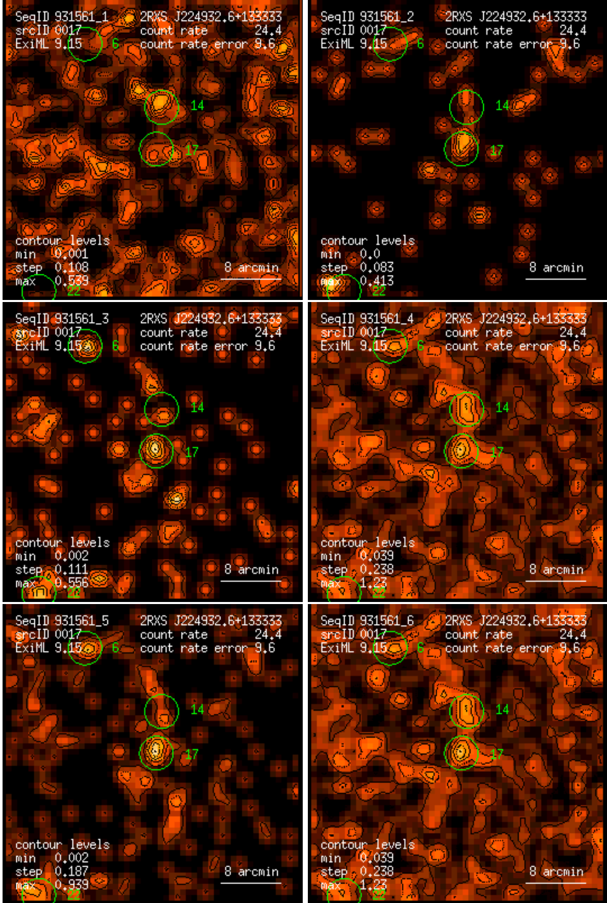
Figure 17: RASS 931561: detection 0017: band rate images, Gaussian filter: (1) PSPC channels 11 – 41, (2) 52 – 90, (3) 91 – 201, (4) 11 – 235, (5) 52 – 201, (6) 11 – 201. Broad band rates in counts/ks. Band rate contour levels in counts/ks/arcmin 2 .
