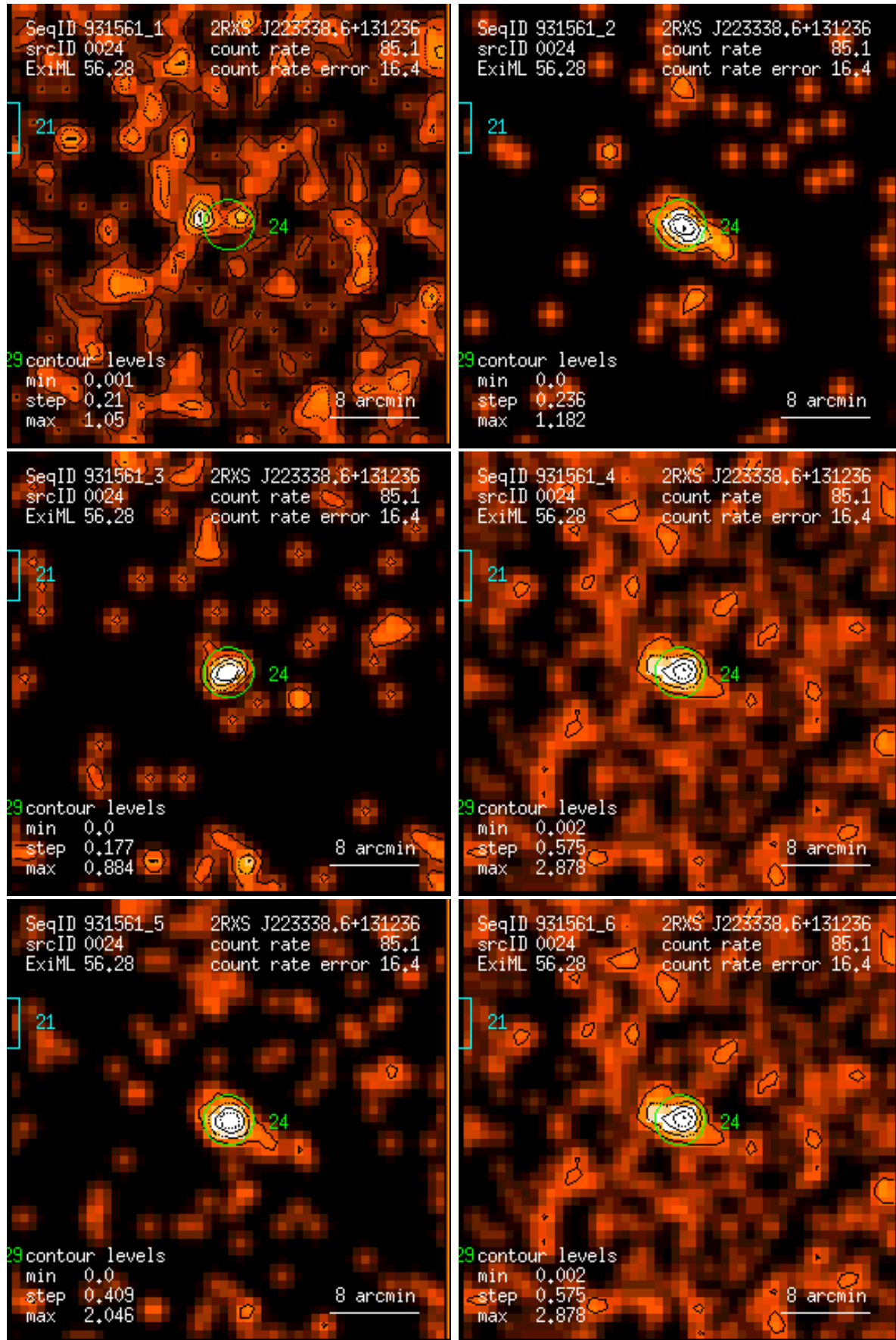
Figure 24: RASS 931561: detection 0024: band rate images, Gaussian filter: (1) PSPC channels 11 – 41, (2) 52 – 90, (3) 91 – 201, (4) 11 – 235, (5) 52 – 201, (6) 11 – 201. Broad band rates in counts/ks. Band rate contour levels in counts/ks/arcmin 2 .
