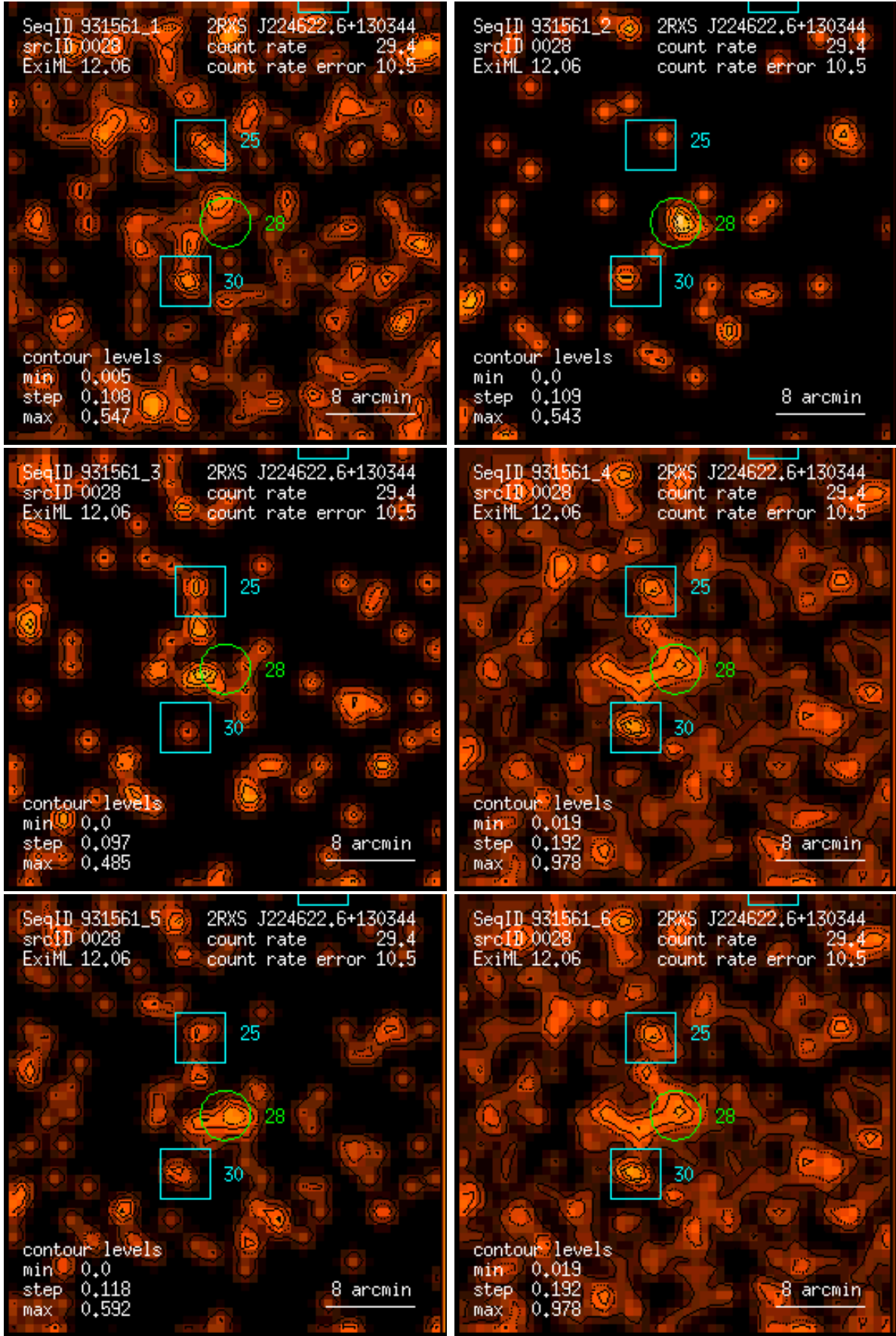
Figure 28: RASS 931561: detection 0028: band rate images, Gaussian filter: (1) PSPC channels 11 – 41, (2) 52 – 90, (3) 91 – 201, (4) 11 – 235, (5) 52 – 201, (6) 11 – 201. Broad band rates in counts/ks. Band rate contour levels in counts/ks/arcmin 2 .
