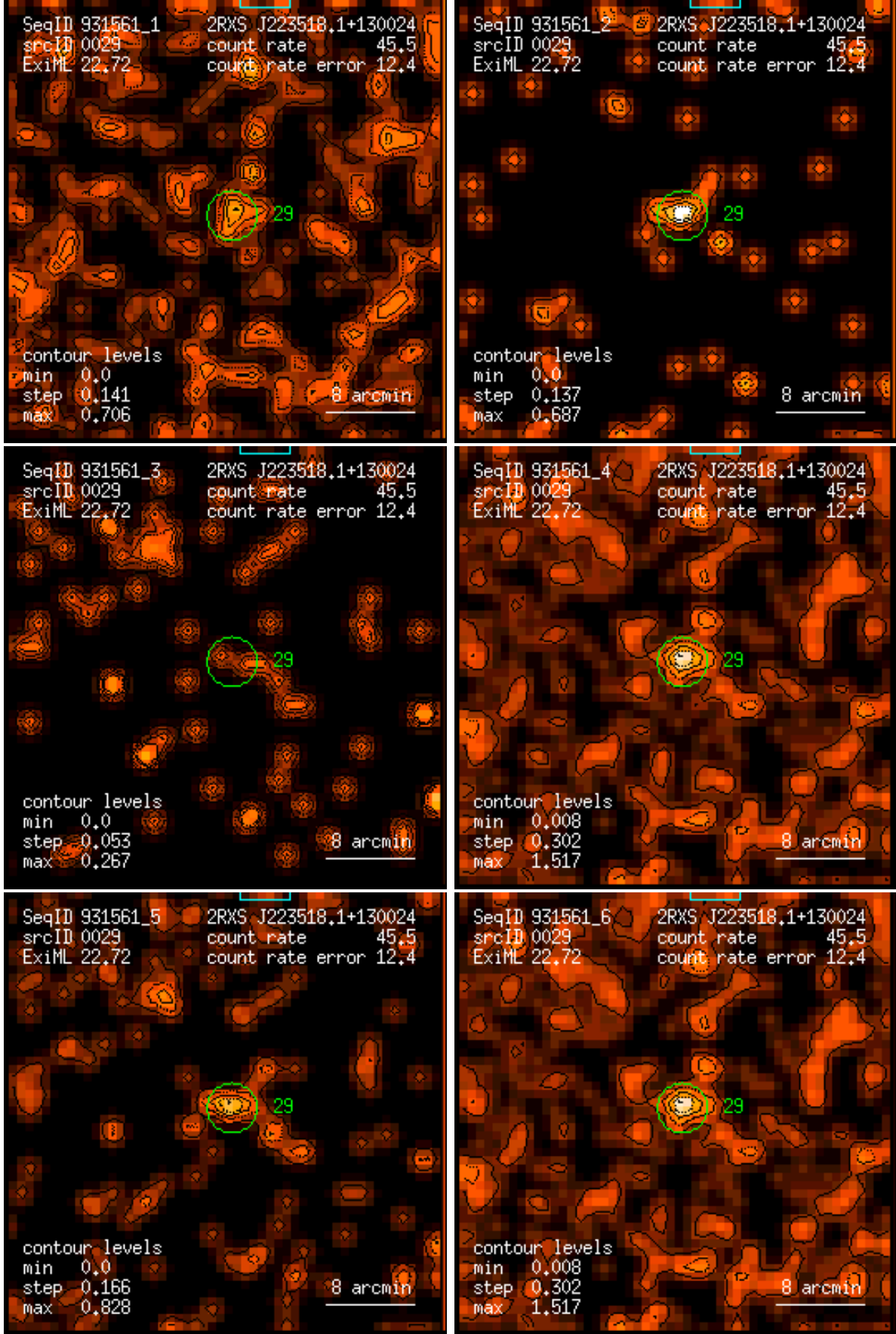
Figure 29: RASS 931561: detection 0029: band rate images, Gaussian filter: (1) PSPC channels 11 – 41, (2) 52 – 90, (3) 91 – 201, (4) 11 – 235, (5) 52 – 201, (6) 11 – 201. Broad band rates in counts/ks. Band rate contour levels in counts/ks/arcmin 2 .
