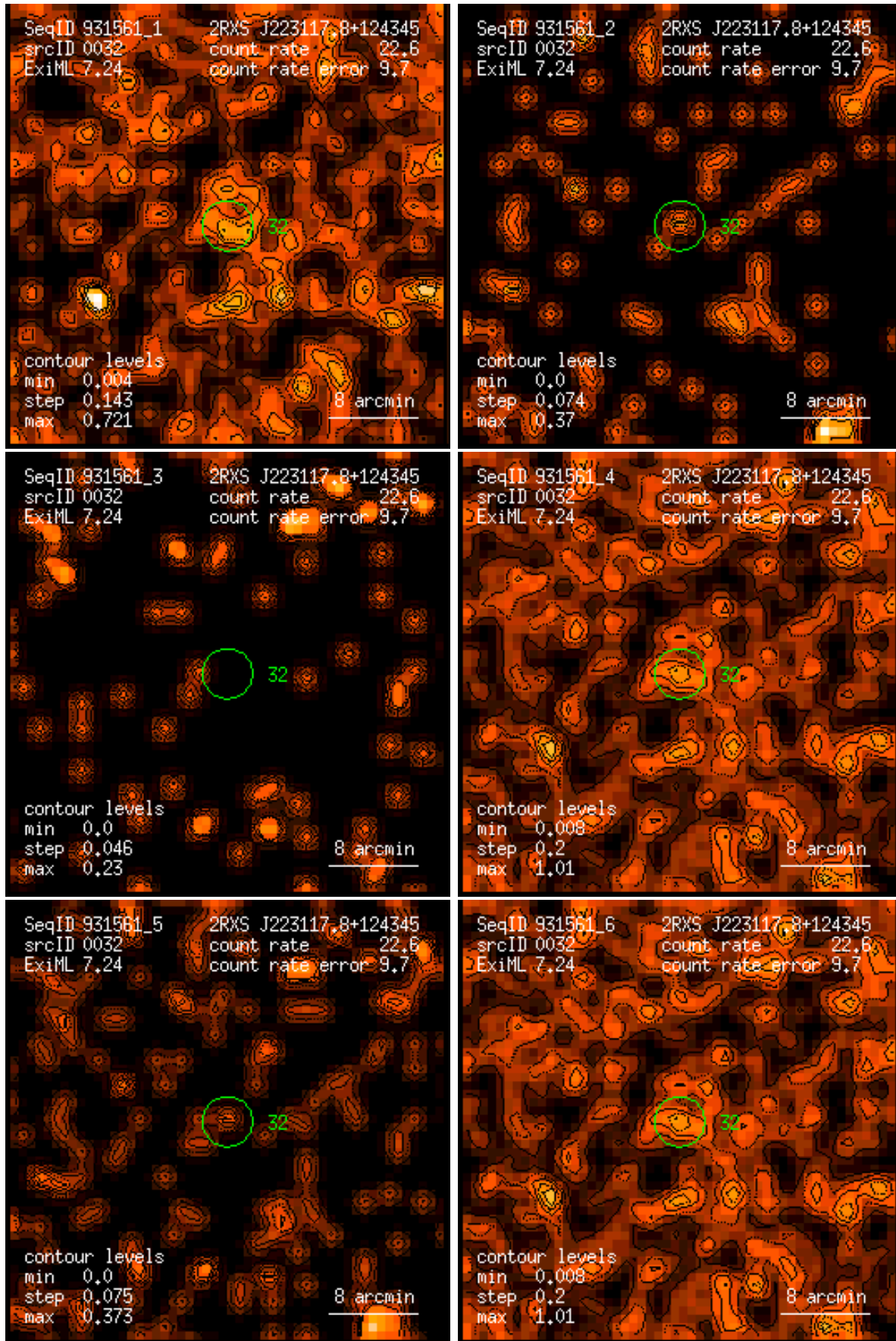
Figure 32: RASS 931561: detection 0032: band rate images, Gaussian filter: (1) PSPC channels 11 – 41, (2) 52 – 90, (3) 91 – 201, (4) 11 – 235, (5) 52 – 201, (6) 11 – 201. Broad band rates in counts/ks. Band rate contour levels in counts/ks/arcmin 2 .
