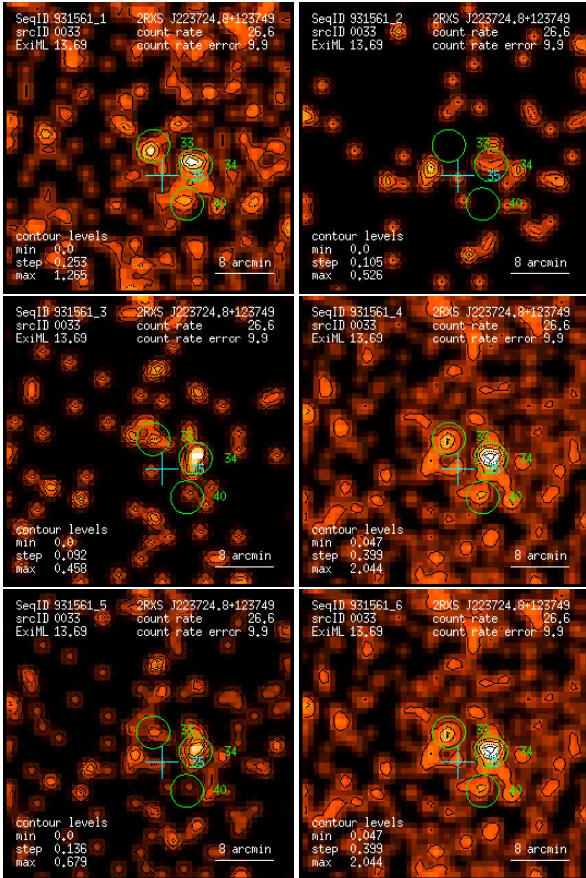
Figure 33: RASS 931561: detection 0033: band rate images, Gaussian filter: (1) PSPC channels 11 – 41, (2) 52 – 90, (3) 91 – 201, (4) 11 – 235, (5) 52 – 201, (6) 11 – 201. Broad band rates in counts/ks. Band rate contour levels in counts/ks/arcmin 2 .
