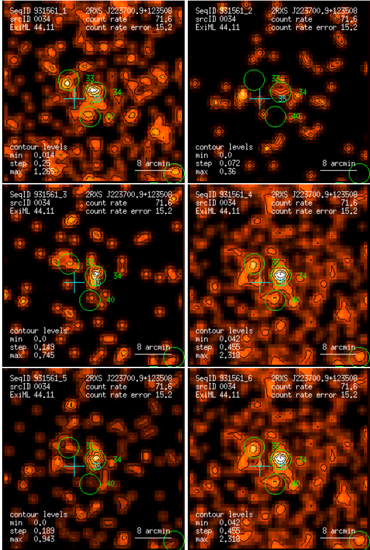
Figure 34: RASS 931561: detection 0034: band rate images, Gaussian filter: (1) PSPC channels 11 – 41, (2) 52 – 90, (3) 91 – 201, (4) 11 – 235, (5) 52 – 201, (6) 11 – 201. Broad band rates in counts/ks. Band rate contour levels in counts/ks/arcmin 2 .
