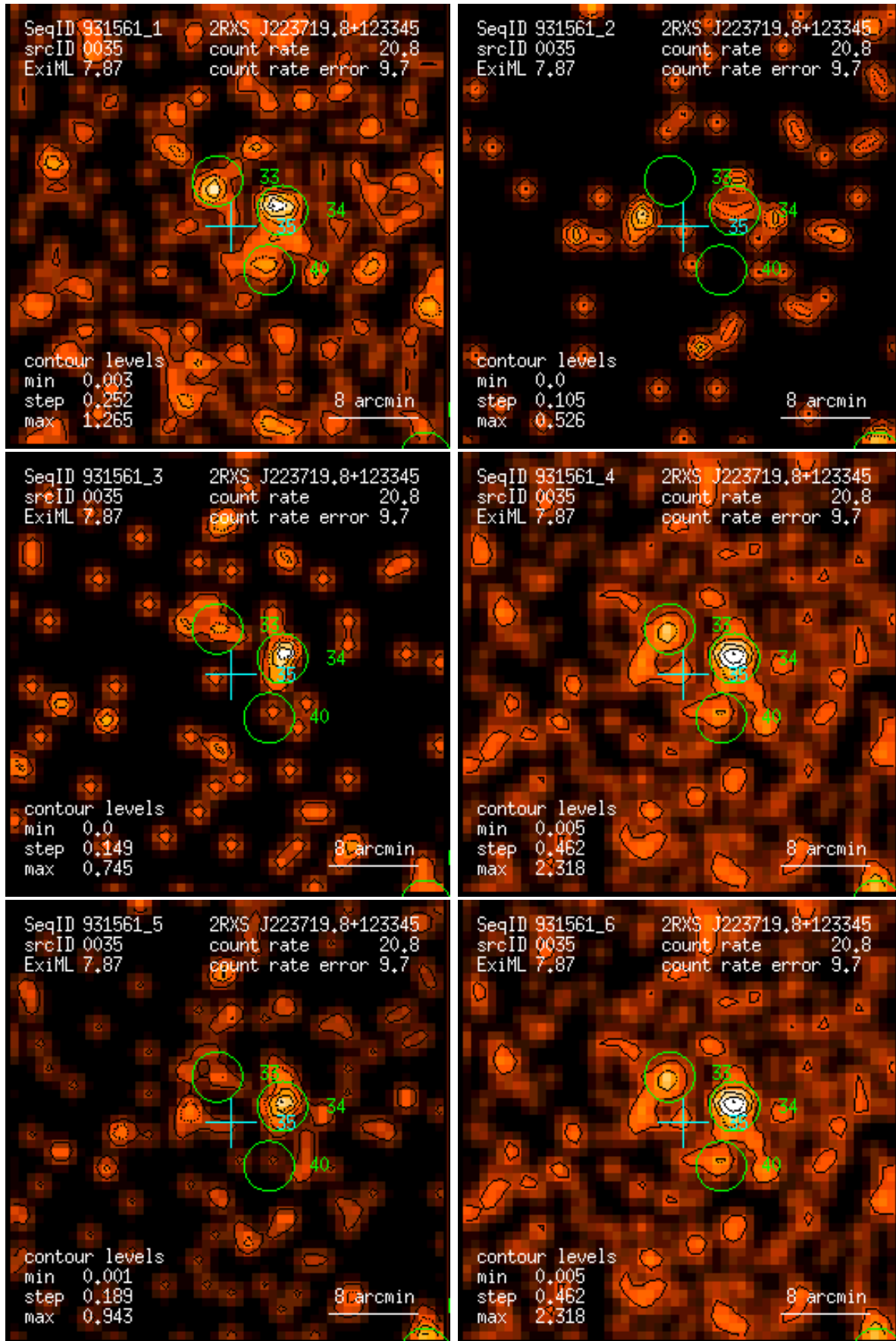
Figure 35: RASS 931561: detection 0035: band rate images, Gaussian filter: (1) PSPC channels 11 – 41, (2) 52 – 90, (3) 91 – 201, (4) 11 – 235, (5) 52 – 201, (6) 11 – 201. Broad band rates in counts/ks. Band rate contour levels in counts/ks/arcmin 2 .
