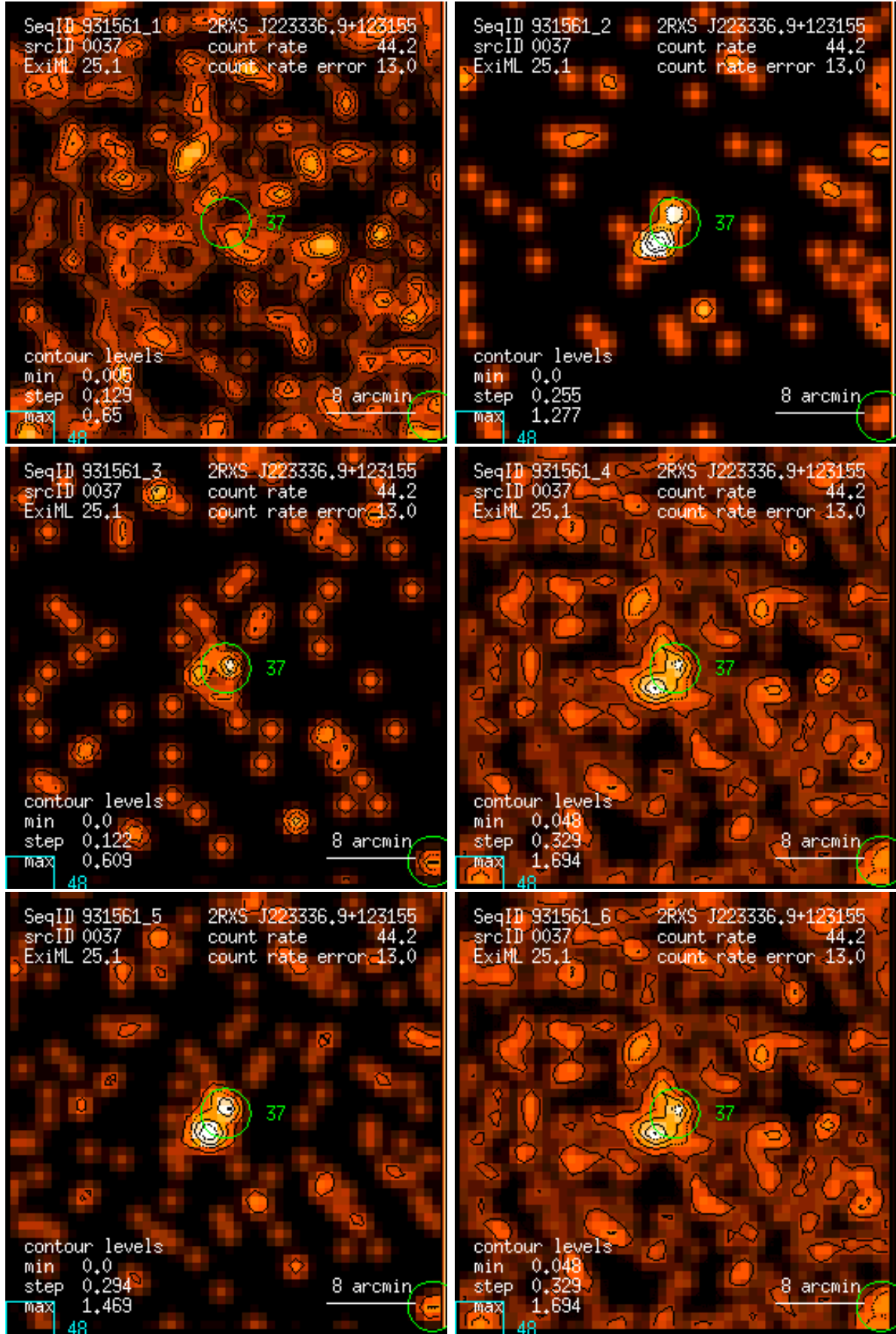
Figure 37: RASS 931561: detection 0037: band rate images, Gaussian filter: (1) PSPC channels 11 – 41, (2) 52 – 90, (3) 91 – 201, (4) 11 – 235, (5) 52 – 201, (6) 11 – 201. Broad band rates in counts/ks. Band rate contour levels in counts/ks/arcmin 2 .
