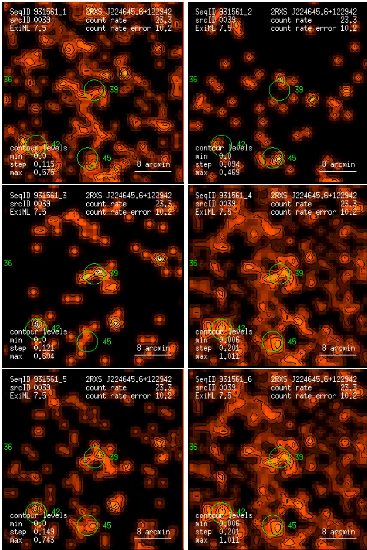
Figure 39: RASS 931561: detection 0039: band rate images, Gaussian filter: (1) PSPC channels 11 – 41, (2) 52 – 90, (3) 91 – 201, (4) 11 – 235, (5) 52 – 201, (6) 11 – 201. Broad band rates in counts/ks. Band rate contour levels in counts/ks/arcmin 2 .
