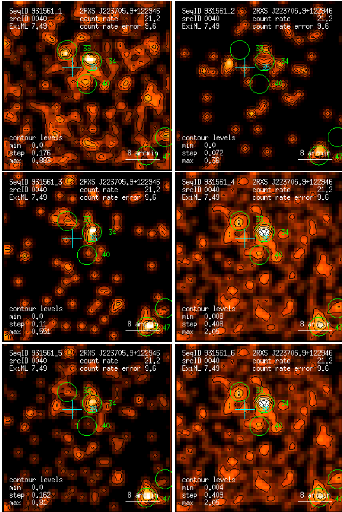
Figure 40: RASS 931561: detection 0040: band rate images, Gaussian filter: (1) PSPC channels 11 – 41, (2) 52 – 90, (3) 91 – 201, (4) 11 – 235, (5) 52 – 201, (6) 11 – 201. Broad band rates in counts/ks. Band rate contour levels in counts/ks/arcmin 2 .
