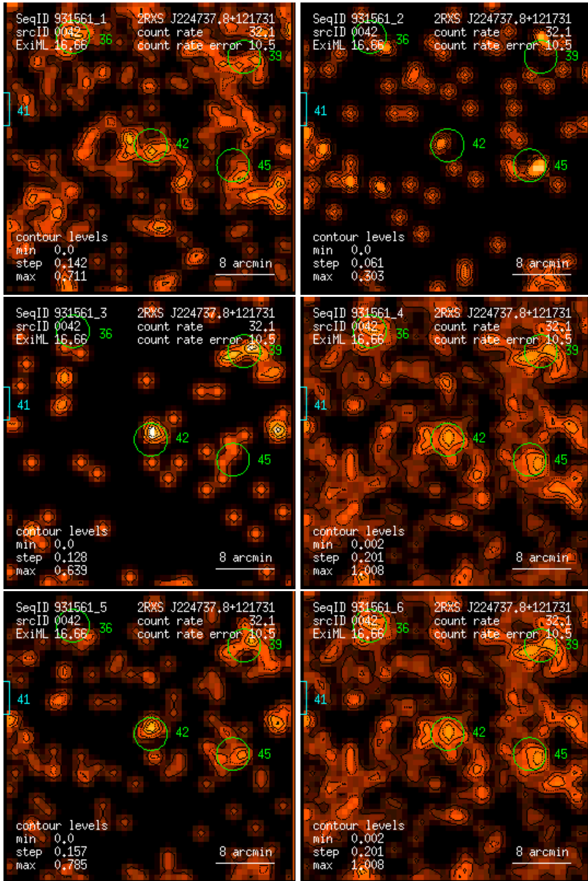
Figure 42: RASS 931561: detection 0042: band rate images, Gaussian filter: (1) PSPC channels 11 – 41, (2) 52 – 90, (3) 91 – 201, (4) 11 – 235, (5) 52 – 201, (6) 11 – 201. Broad band rates in counts/ks. Band rate contour levels in counts/ks/arcmin 2 .
