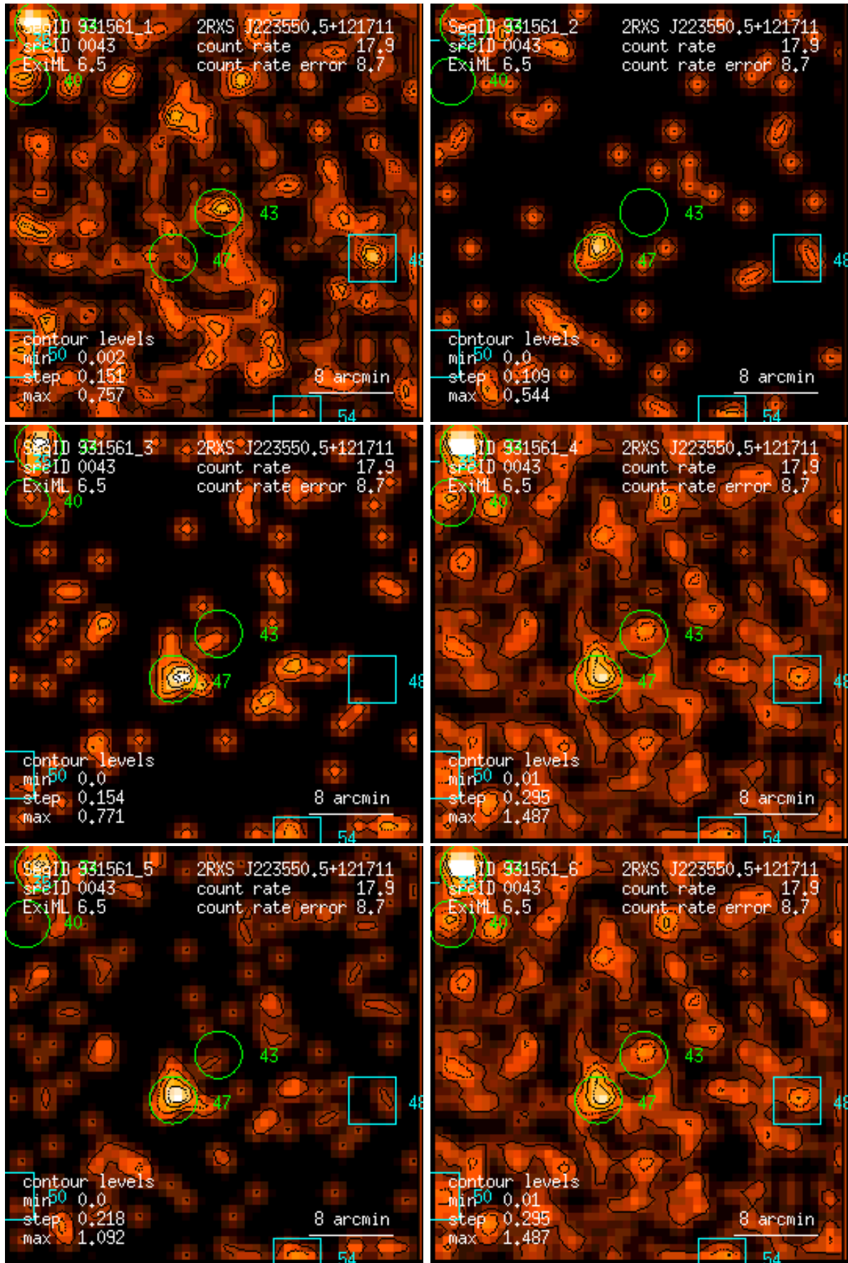
Figure 43: RASS 931561: detection 0043: band rate images, Gaussian filter: (1) PSPC channels 11 – 41, (2) 52 – 90, (3) 91 – 201, (4) 11 – 235, (5) 52 – 201, (6) 11 – 201. Broad band rates in counts/ks. Band rate contour levels in counts/ks/arcmin 2 .
