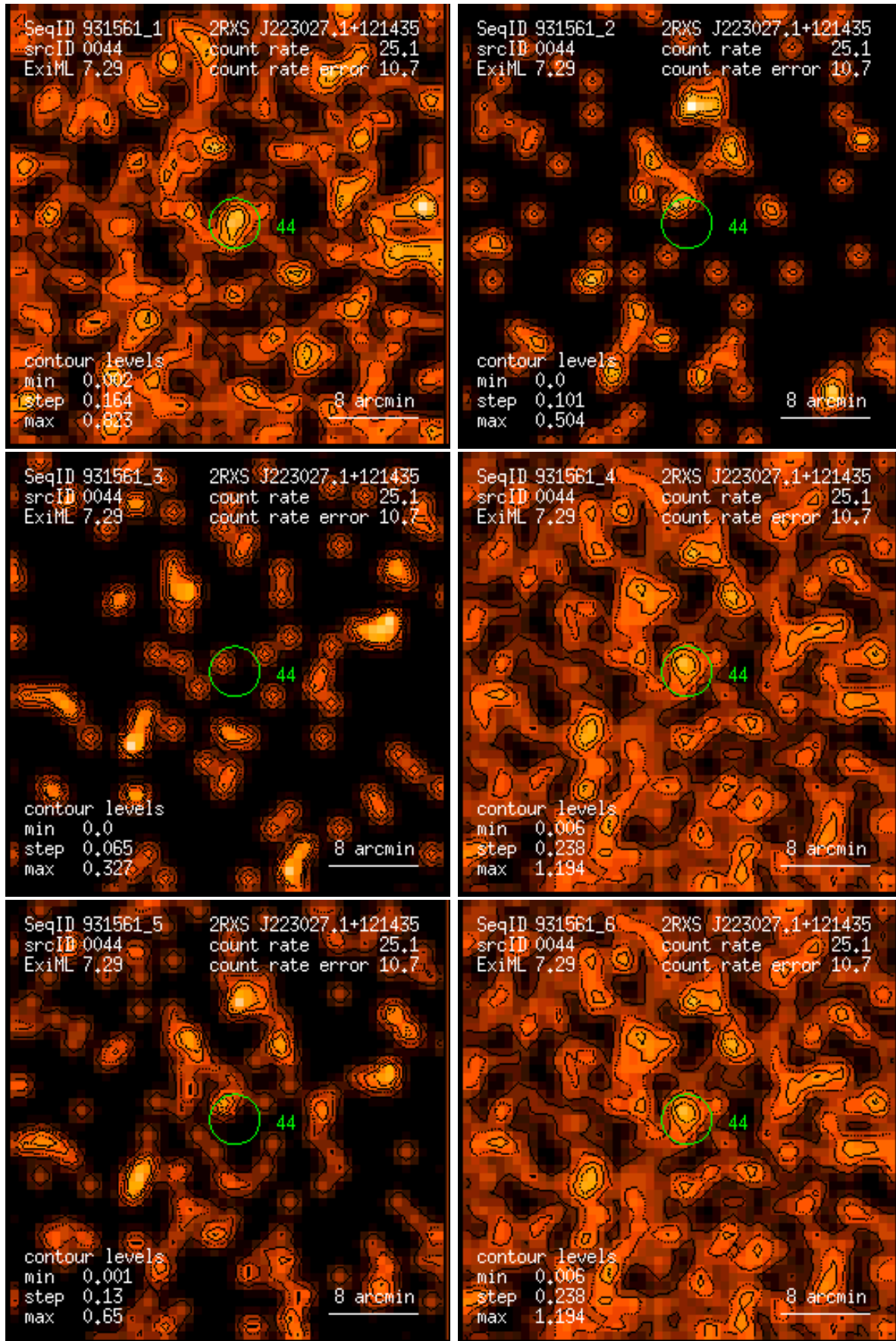
Figure 44: RASS 931561: detection 0044: band rate images, Gaussian filter: (1) PSPC channels 11 – 41, (2) 52 – 90, (3) 91 – 201, (4) 11 – 235, (5) 52 – 201, (6) 11 – 201. Broad band rates in counts/ks. Band rate contour levels in counts/ks/arcmin 2 .
