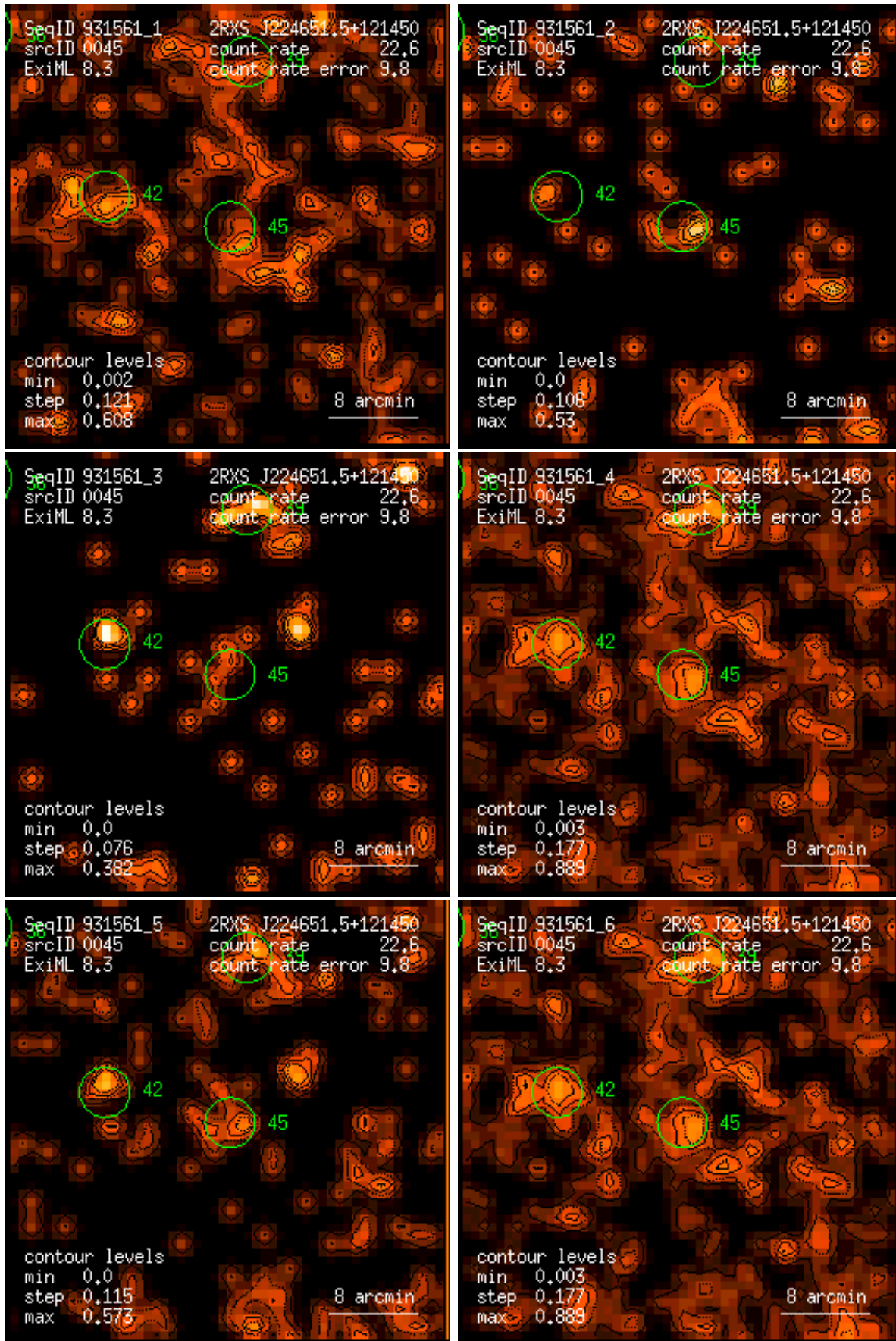
Figure 45: RASS 931561: detection 0045: band rate images, Gaussian filter: (1) PSPC channels 11 – 41, (2) 52 – 90, (3) 91 – 201, (4) 11 – 235, (5) 52 – 201, (6) 11 – 201. Broad band rates in counts/ks. Band rate contour levels in counts/ks/arcmin 2 .
