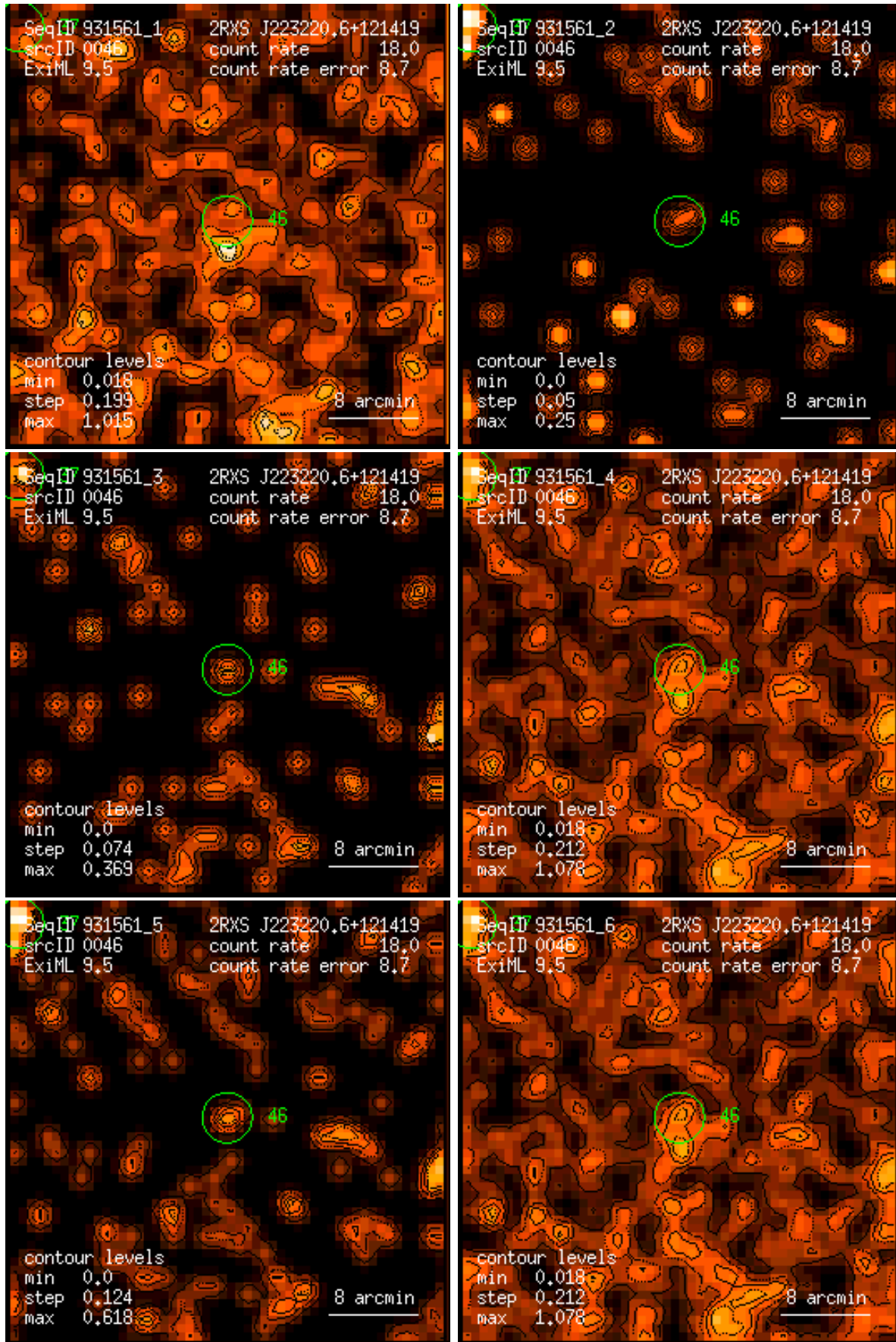
Figure 46: RASS 931561: detection 0046: band rate images, Gaussian filter: (1) PSPC channels 11 – 41, (2) 52 – 90, (3) 91 – 201, (4) 11 – 235, (5) 52 – 201, (6) 11 – 201. Broad band rates in counts/ks. Band rate contour levels in counts/ks/arcmin 2 .
