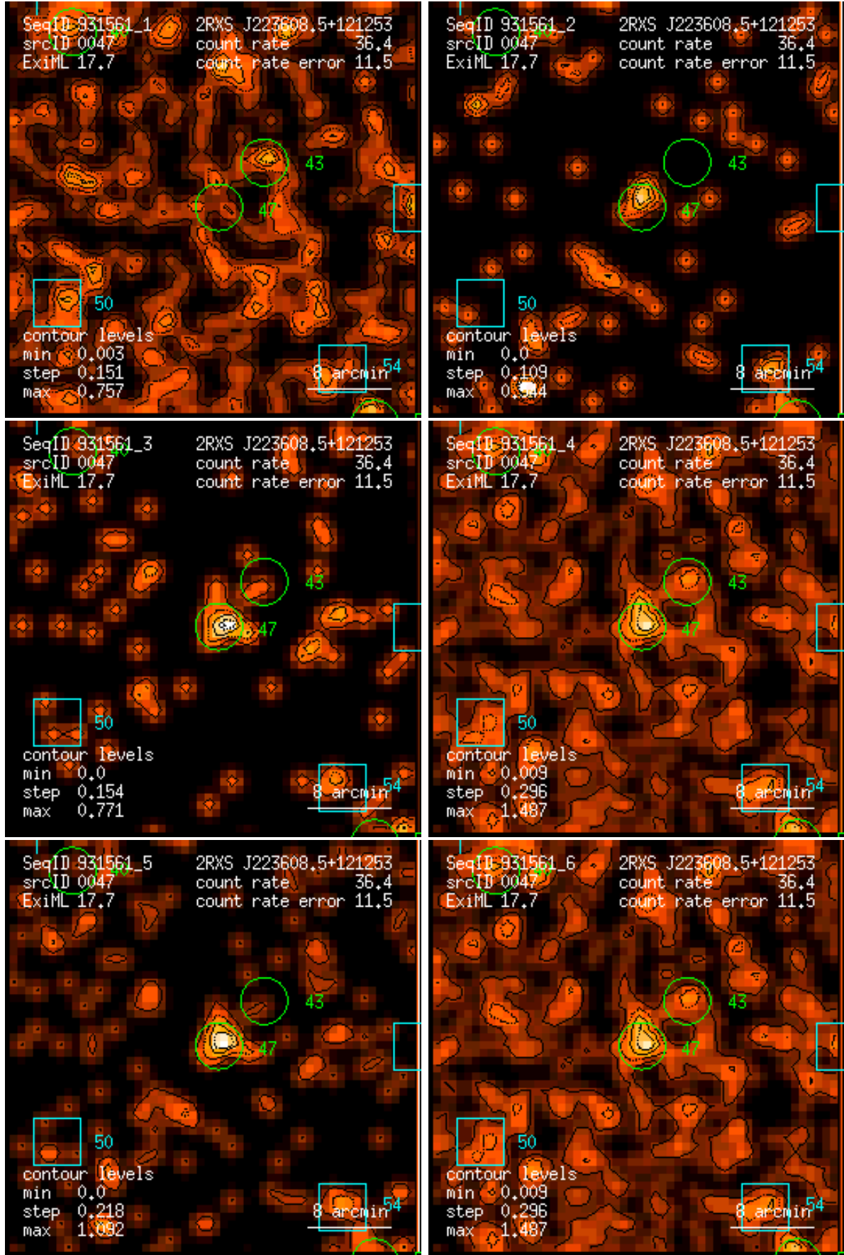
Figure 47: RASS 931561: detection 0047: band rate images, Gaussian filter: (1) PSPC channels 11 – 41, (2) 52 – 90, (3) 91 – 201, (4) 11 – 235, (5) 52 – 201, (6) 11 – 201. Broad band rates in counts/ks. Band rate contour levels in counts/ks/arcmin 2 .
