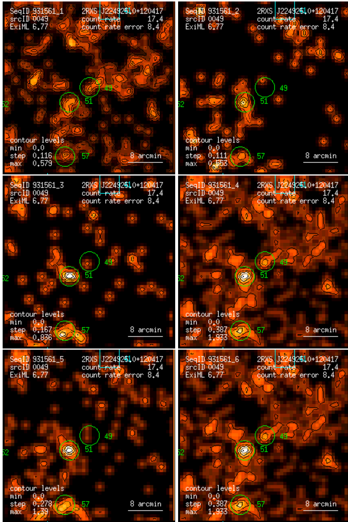
Figure 49: RASS 931561: detection 0049: band rate images, Gaussian filter: (1) PSPC channels 11 – 41, (2) 52 – 90, (3) 91 – 201, (4) 11 – 235, (5) 52 – 201, (6) 11 – 201. Broad band rates in counts/ks. Band rate contour levels in counts/ks/arcmin 2 .
