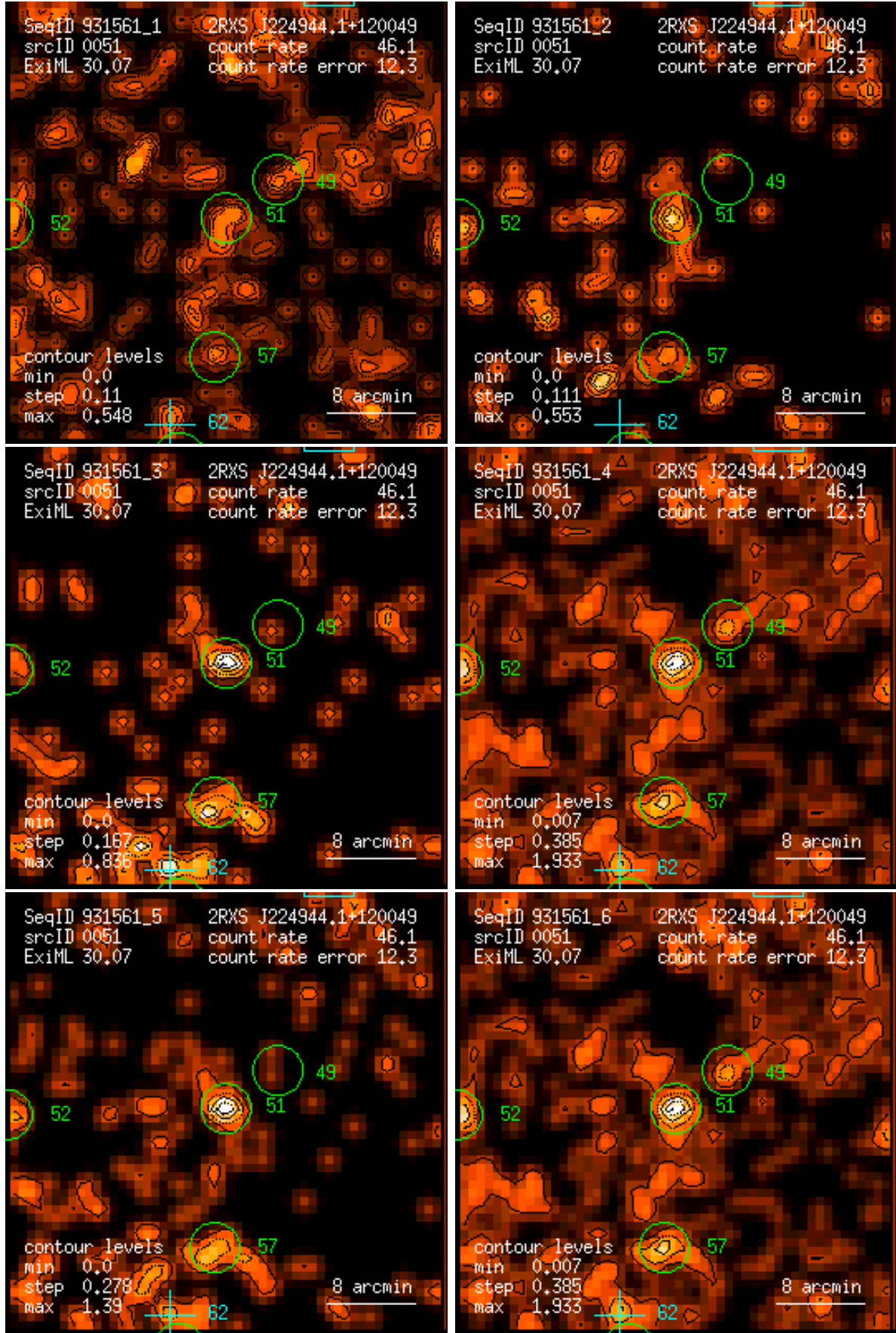
Figure 51: RASS 931561: detection 0051: band rate images, Gaussian filter: (1) PSPC channels 11 – 41, (2) 52 – 90, (3) 91 – 201, (4) 11 – 235, (5) 52 – 201, (6) 11 – 201. Broad band rates in counts/ks. Band rate contour levels in counts/ks/arcmin 2 .
