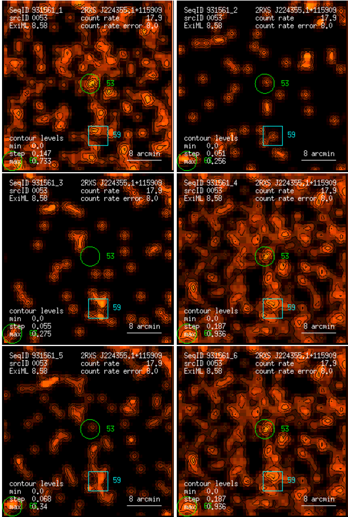
Figure 53: RASS 931561: detection 0053: band rate images, Gaussian filter: (1) PSPC channels 11 – 41, (2) 52 – 90, (3) 91 – 201, (4) 11 – 235, (5) 52 – 201, (6) 11 – 201. Broad band rates in counts/ks. Band rate contour levels in counts/ks/arcmin 2 .
