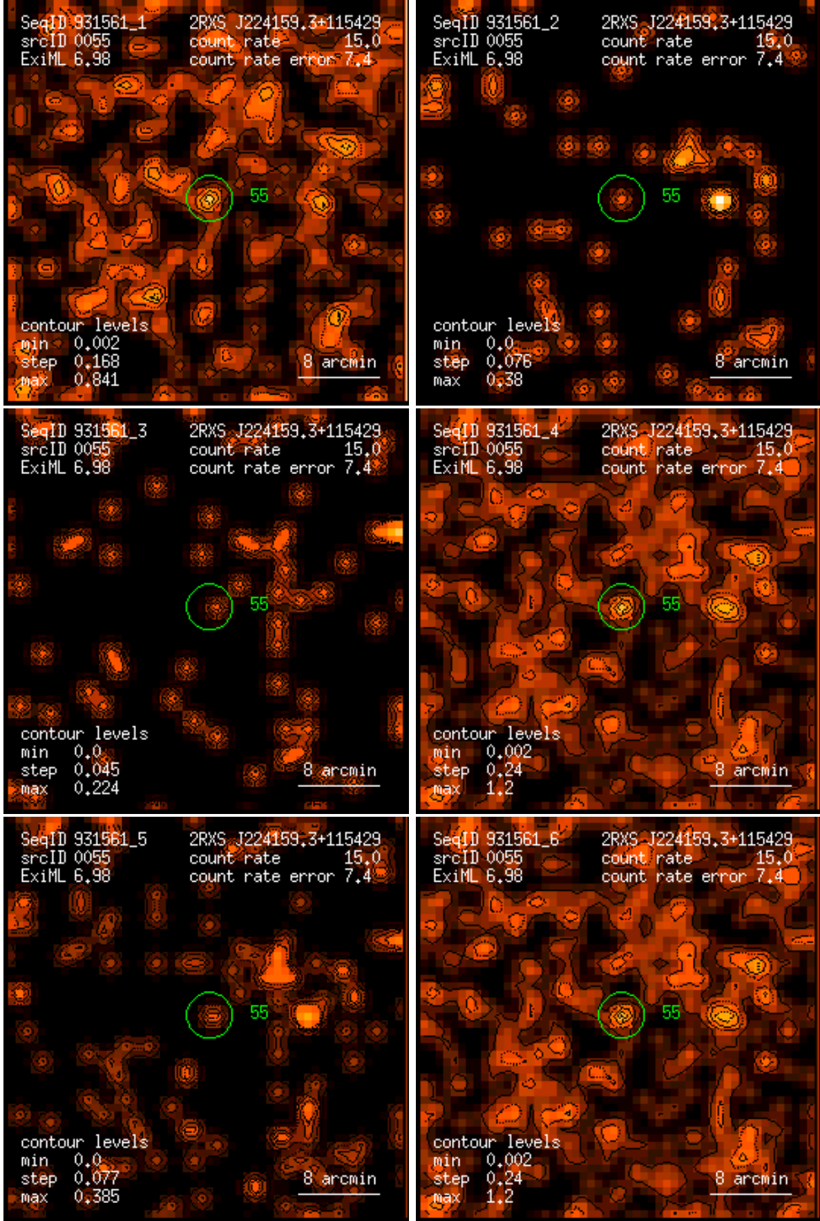
Figure 55: RASS 931561: detection 0055: band rate images, Gaussian filter: (1) PSPC channels 11 – 41, (2) 52 – 90, (3) 91 – 201, (4) 11 – 235, (5) 52 – 201, (6) 11 – 201. Broad band rates in counts/ks. Band rate contour levels in counts/ks/arcmin 2 .
