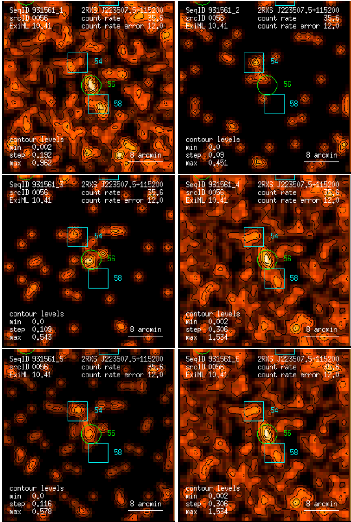
Figure 56: RASS 931561: detection 0056: band rate images, Gaussian filter: (1) PSPC channels 11 – 41, (2) 52 – 90, (3) 91 – 201, (4) 11 – 235, (5) 52 – 201, (6) 11 – 201. Broad band rates in counts/ks. Band rate contour levels in counts/ks/arcmin 2 .
