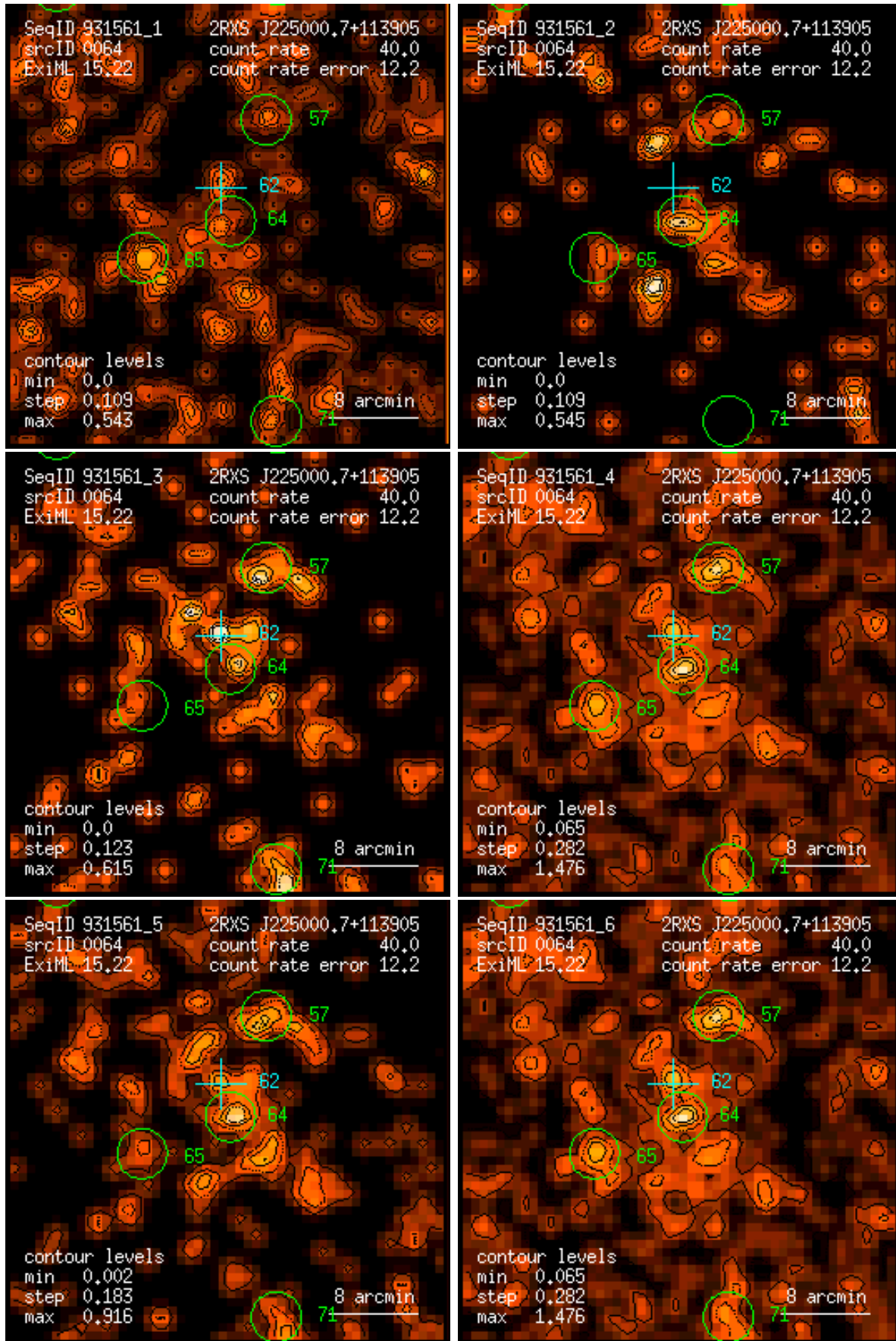
Figure 64: RASS 931561: detection 0064: band rate images, Gaussian filter: (1) PSPC channels 11 – 41, (2) 52 – 90, (3) 91 – 201, (4) 11 – 235, (5) 52 – 201, (6) 11 – 201. Broad band rates in counts/ks. Band rate contour levels in counts/ks/arcmin 2 .
