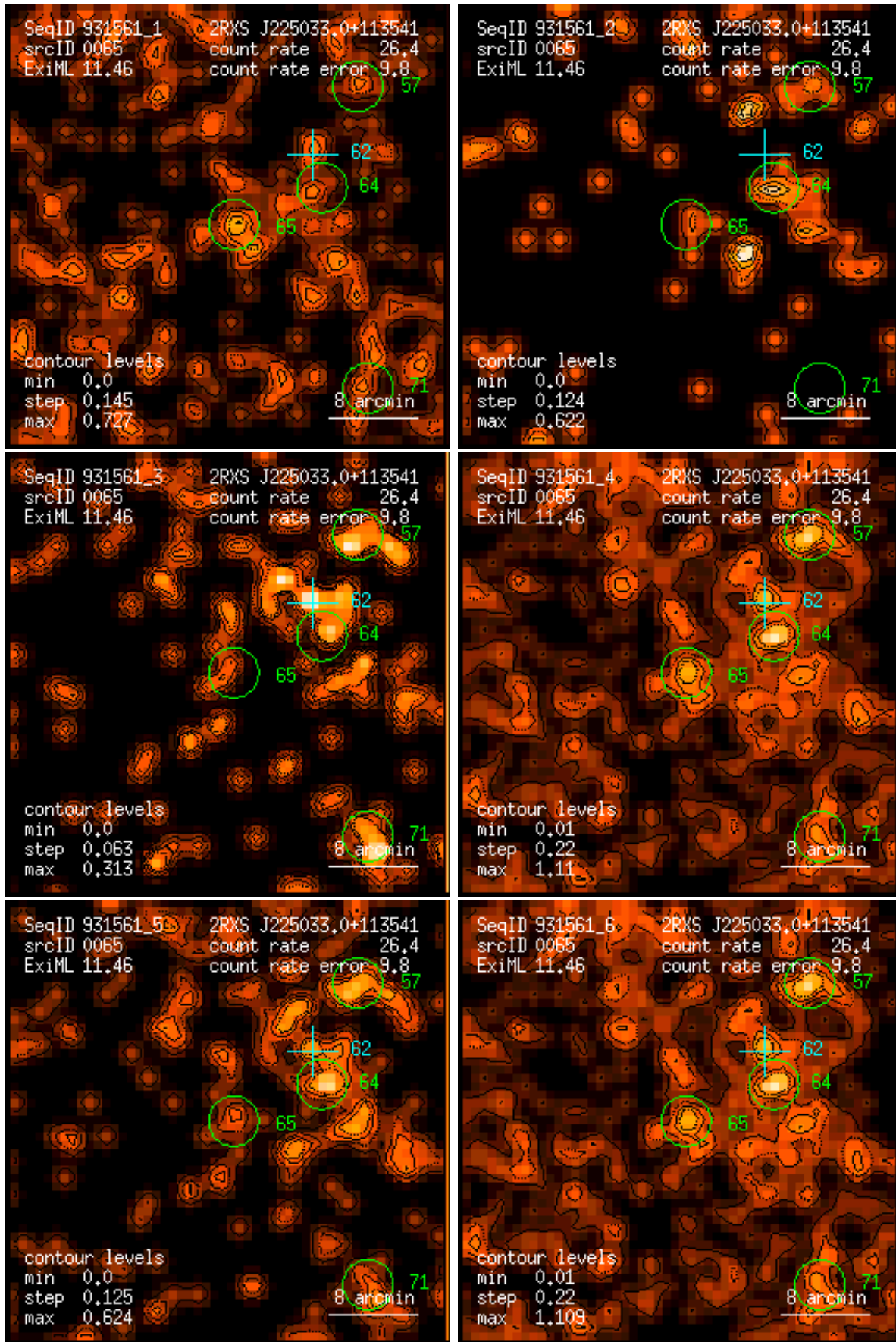
Figure 65: RASS 931561: detection 0065: band rate images, Gaussian filter: (1) PSPC channels 11 – 41, (2) 52 – 90, (3) 91 – 201, (4) 11 – 235, (5) 52 – 201, (6) 11 – 201. Broad band rates in counts/ks. Band rate contour levels in counts/ks/arcmin 2 .
