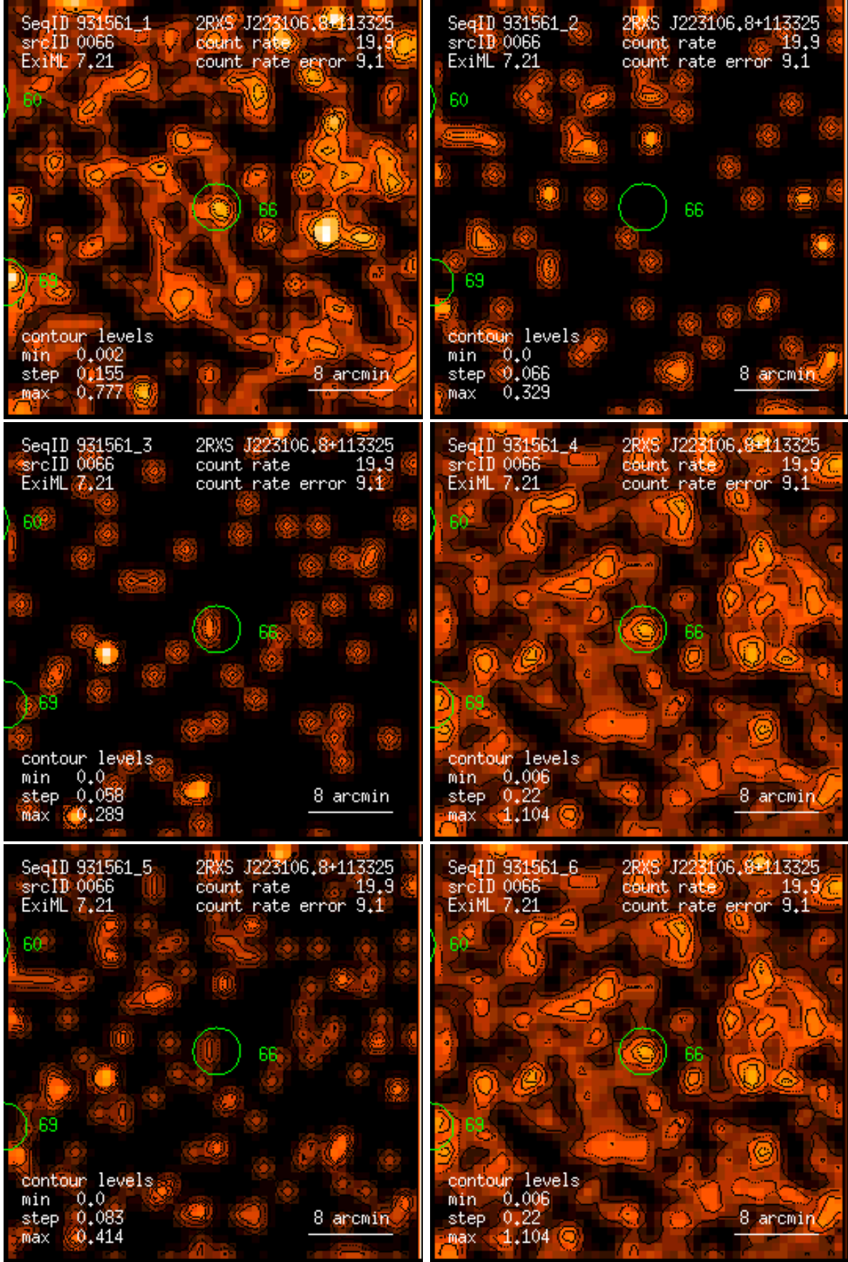
Figure 66: RASS 931561: detection 0066: band rate images, Gaussian filter: (1) PSPC channels 11 – 41, (2) 52 – 90, (3) 91 – 201, (4) 11 – 235, (5) 52 – 201, (6) 11 – 201. Broad band rates in counts/ks. Band rate contour levels in counts/ks/arcmin 2 .
