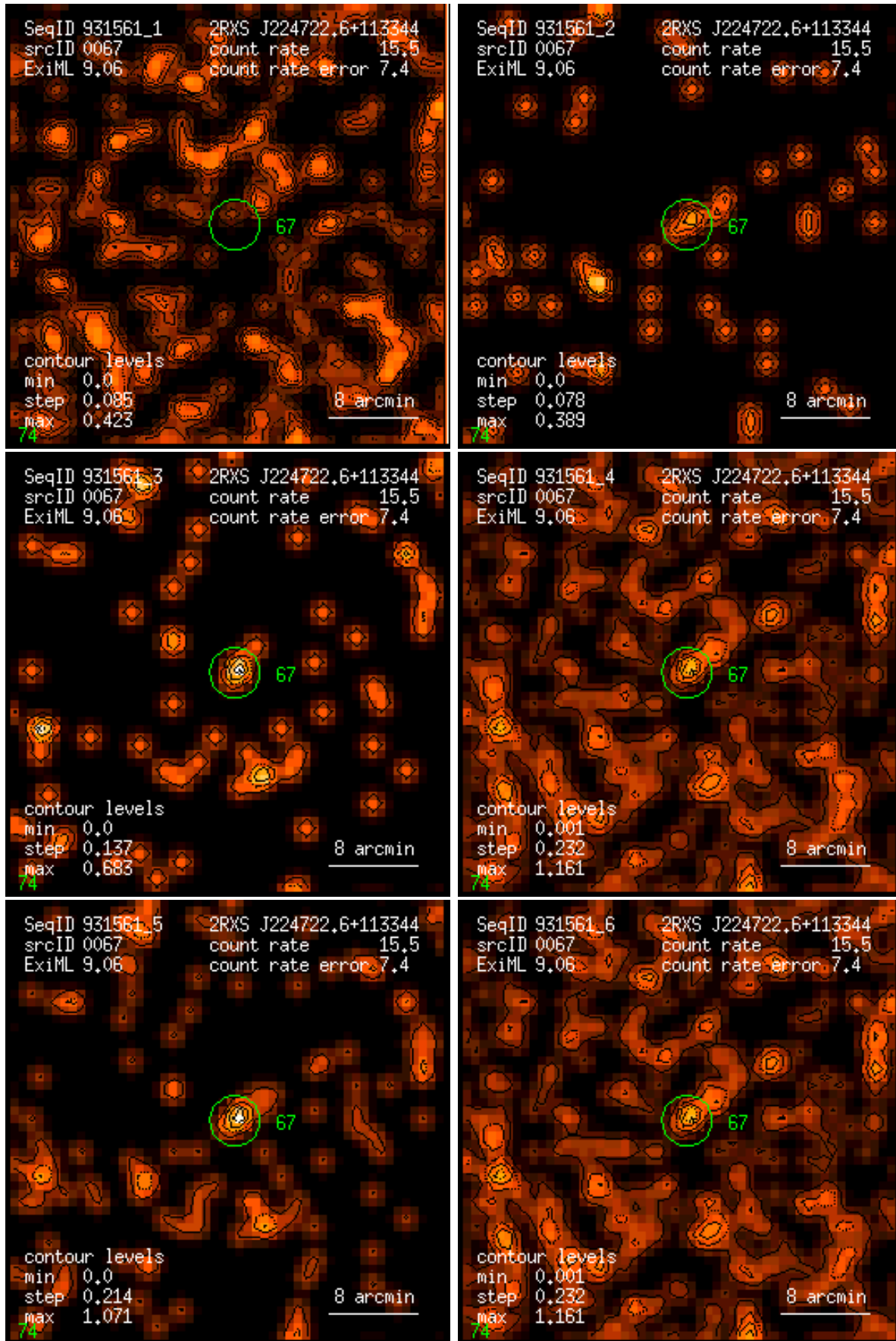
Figure 67: RASS 931561: detection 0067: band rate images, Gaussian filter: (1) PSPC channels 11 – 41, (2) 52 – 90, (3) 91 – 201, (4) 11 – 235, (5) 52 – 201, (6) 11 – 201. Broad band rates in counts/ks. Band rate contour levels in counts/ks/arcmin 2 .
