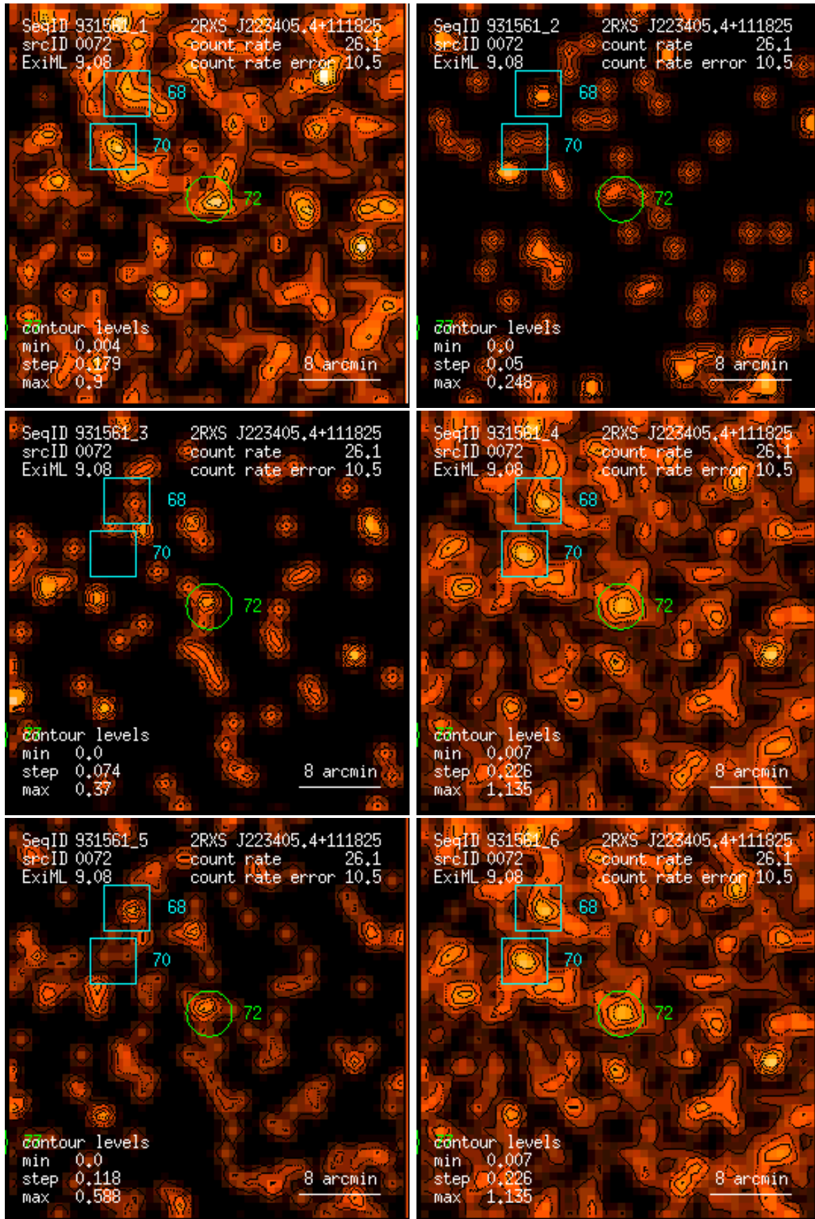
Figure 72: RASS 931561: detection 0072: band rate images, Gaussian filter: (1) PSPC channels 11 – 41, (2) 52 – 90, (3) 91 – 201, (4) 11 – 235, (5) 52 – 201, (6) 11 – 201. Broad band rates in counts/ks. Band rate contour levels in counts/ks/arcmin 2 .
