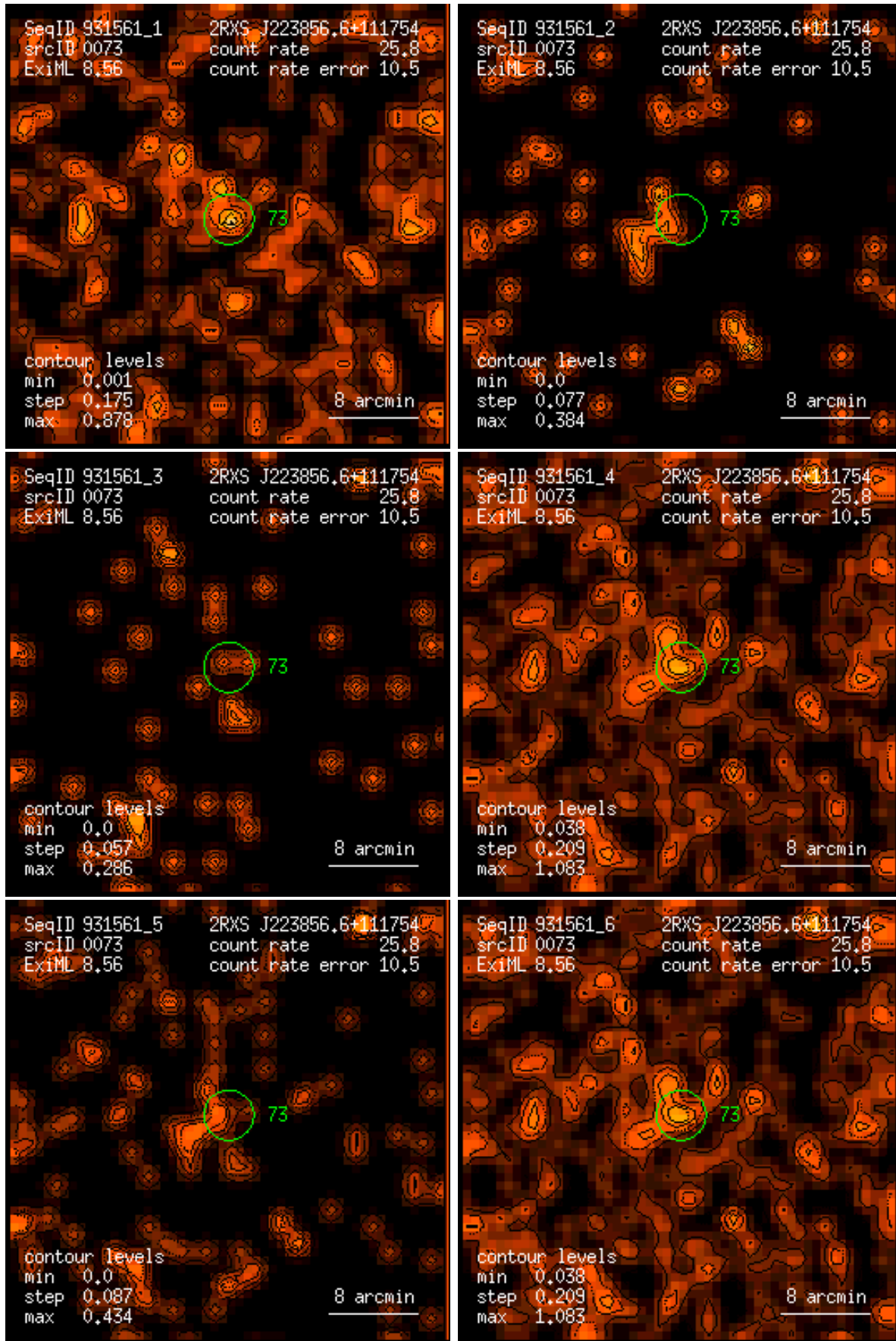
Figure 73: RASS 931561: detection 0073: band rate images, Gaussian filter: (1) PSPC channels 11 – 41, (2) 52 – 90, (3) 91 – 201, (4) 11 – 235, (5) 52 – 201, (6) 11 – 201. Broad band rates in counts/ks. Band rate contour levels in counts/ks/arcmin 2 .
